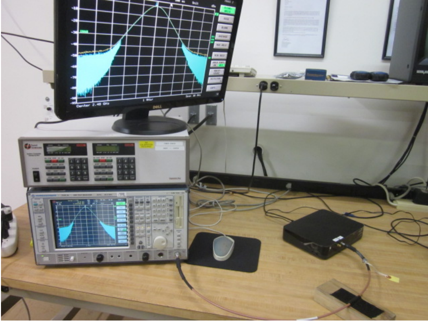
Conducted Emissions Antenna Test Setup Picture
