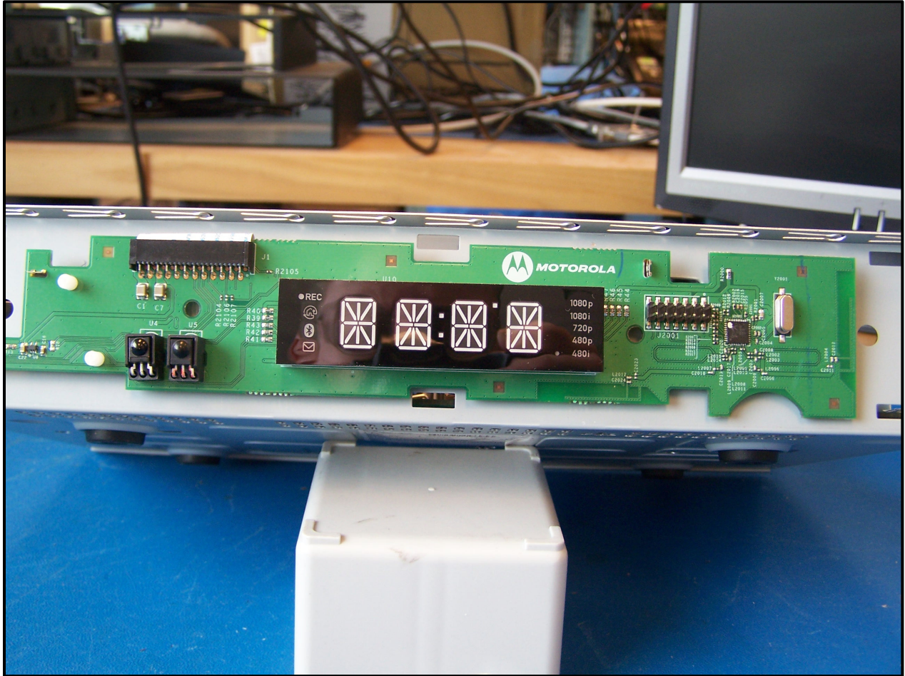
Photograph 11: RF Board – Front View
