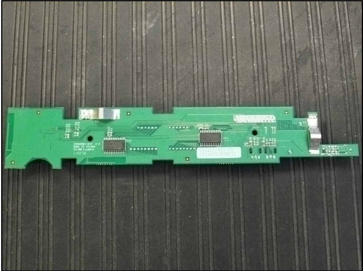
Photograph 13: RF Board – Back View
