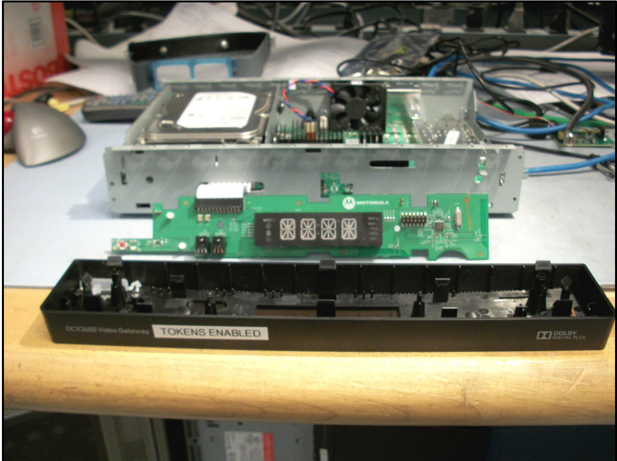
Photograph 10: RF Board with Chassis
