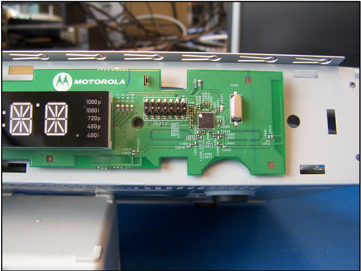
Photograph 12: RF Board – Front View Partial - Close Up
