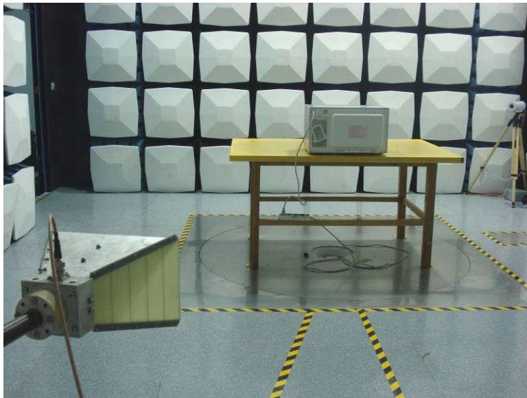
Radiated Emissions - Rear View (Above 1 GHz)
