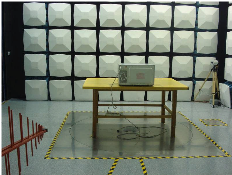
Radiated Emissions - Rear View (Below 1 GHz)
