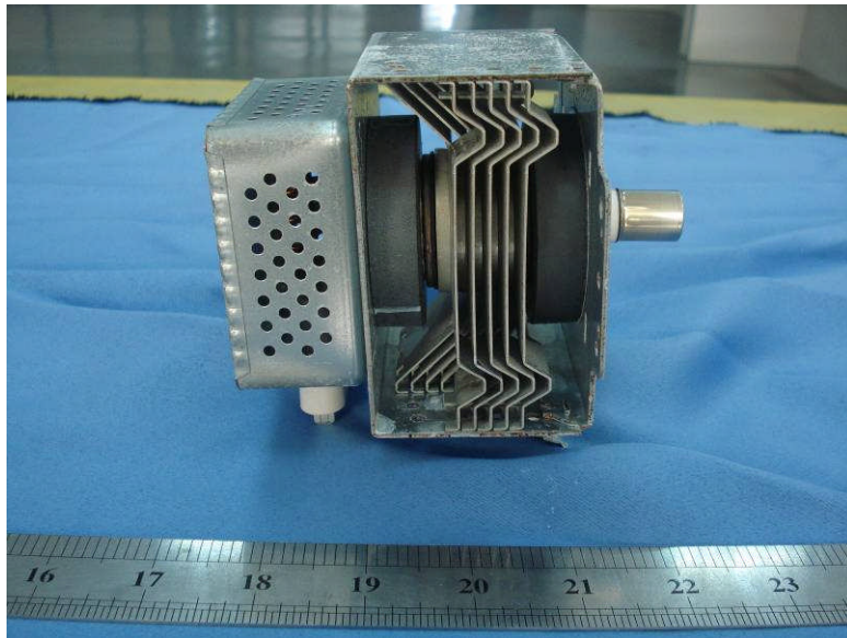
EUT – Magnetron Side View
