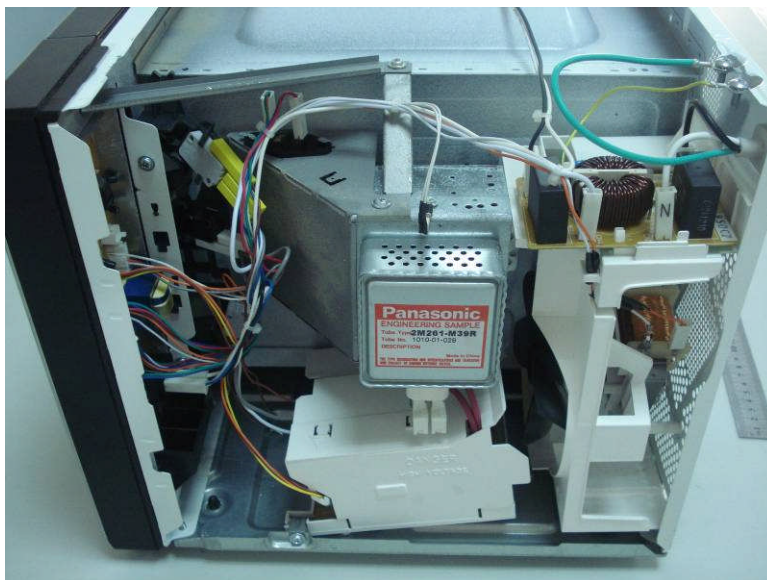
EUT – Uncovered 2 View
