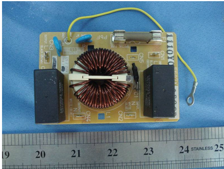
EUT – Filter Board Front View
