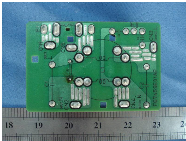
EUT – Filter Board Rear View
