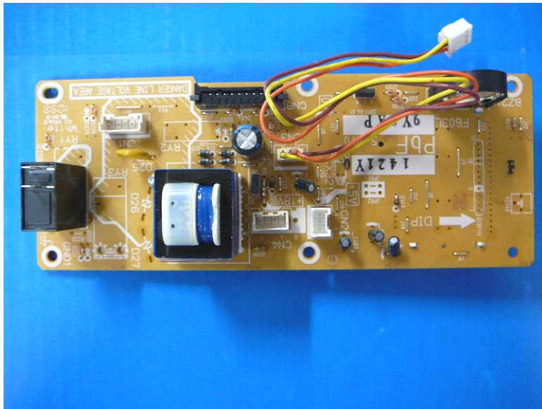
EUT – Control Board Front View
