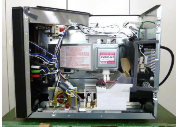
Right Side View With Enclosure Removed
