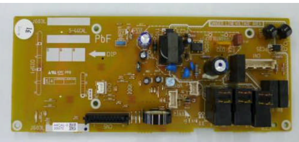
View of Controller
