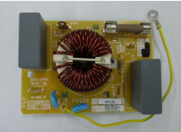
View of Power Line Filter
