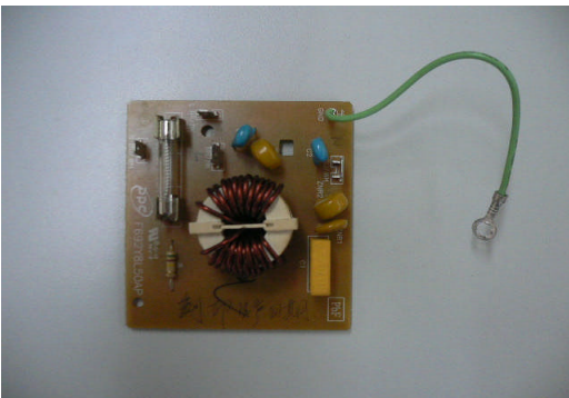
Exhibit: B5 View of Power Line Filter Circuitry
