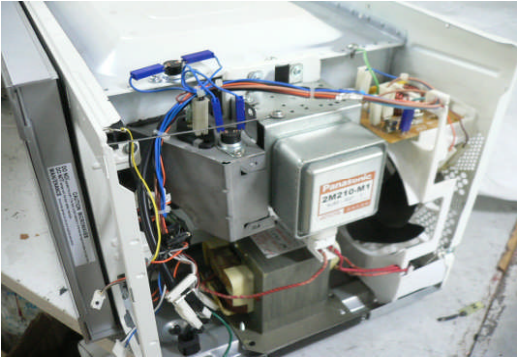
Exhibit: B3 NN-SD377 Right side view, No enclosure
