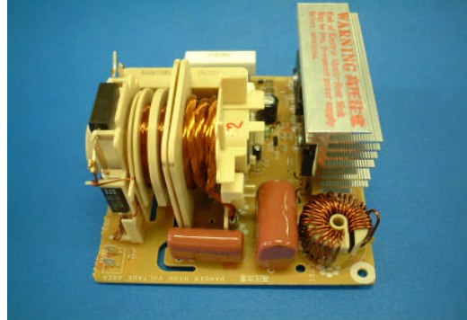
Exhibit: B4 View of Inverter Circuitry (Power Supply)
