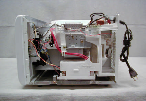
Exhibit: B3 NN-H665 Right side view, No enclosure
