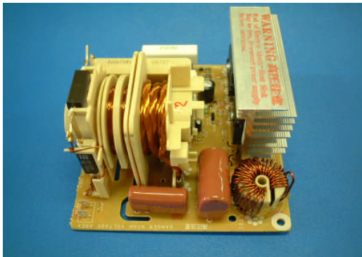
Exhibit: B5 View of Inverter Circuitry (Power Supply)
