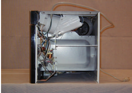
Exhibit: B3 Right side view, No enclosure NN-P295SF
