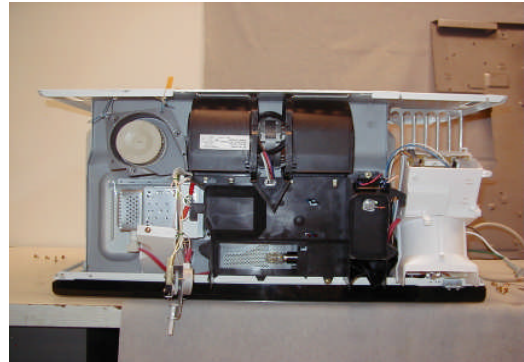
Exhibit: B4 Top view, No enclosure NN-P295SF
