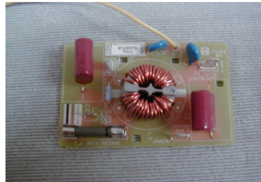
Exhibit: B6 View of Power Line Filter Circuitry
