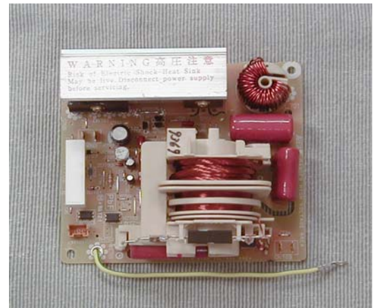
Exhibit 2-K View of Inverter (
