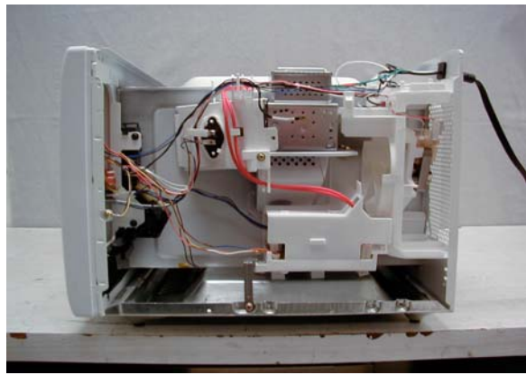
Exhibit 2-D2 Right side view No enclosure NN-S954WF
