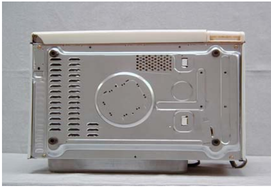
Exhibit 2-G Bottom view NN-S443WF
