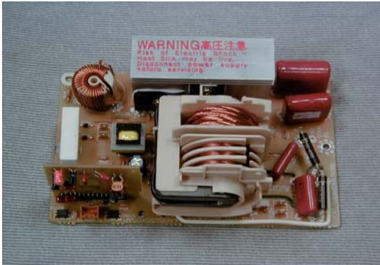
Exhibit 2-K View of Inverter Circuitry
