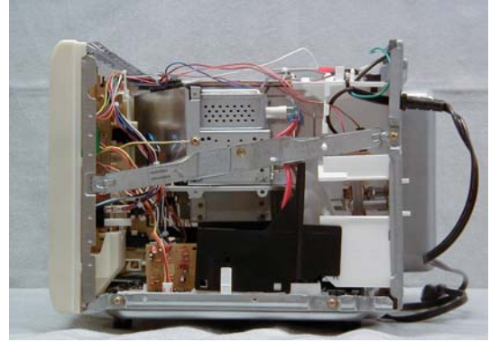
Exhibit 2-D2 Right side view, No enclosure NN-G463WF
