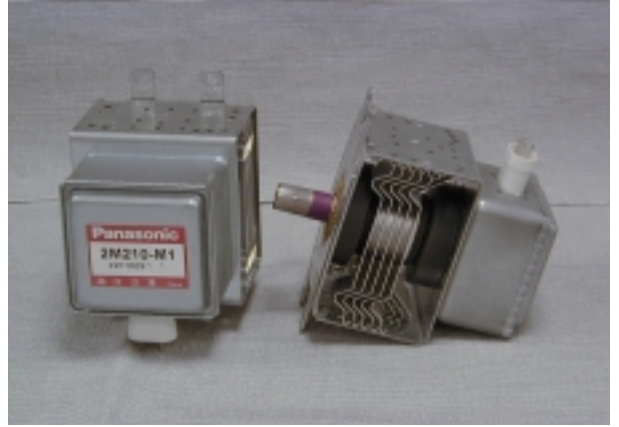
Exhibit 2-H Magnetron 2M-210-M1
