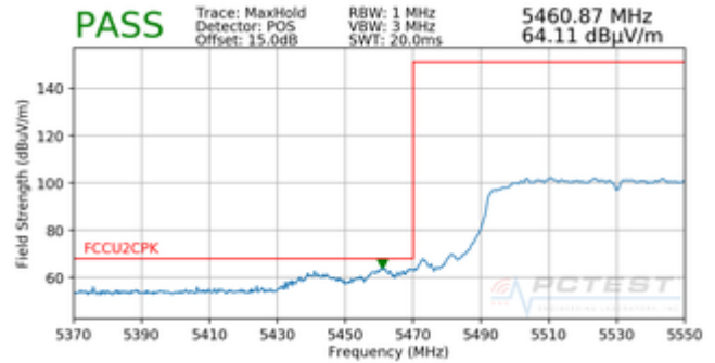
Plot 7-109. Radiated Lower Band Edge Plot (Peak – UNII Band 2C)
