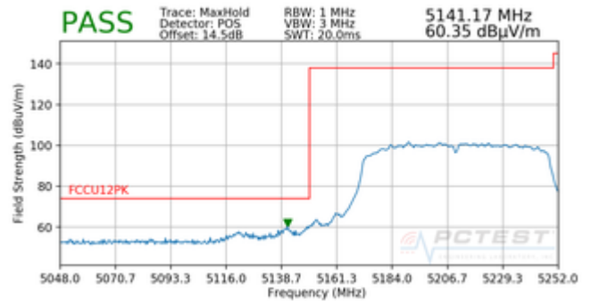
Plot 7-105. Radiated Lower Band Edge Plot (Peak – UNII Band 1)
