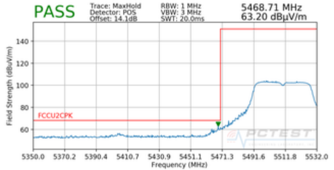
Plot 7-98. Radiated Lower Band Edge Plot (Peak – UNII Band 2C)
