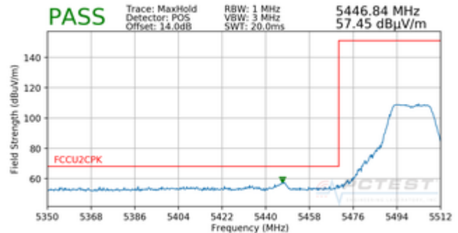
Plot 7-92. Radiated Band Edge Plot (Peak – Rugged USB Dock)
