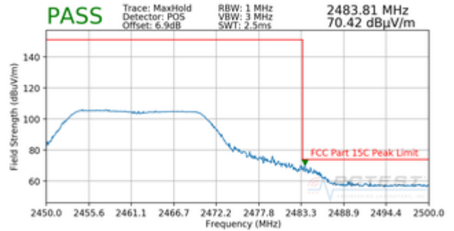
Plot 7-40. Radiated Restricted Band Edge Measurement with Rugged USB Dock (Peak)
