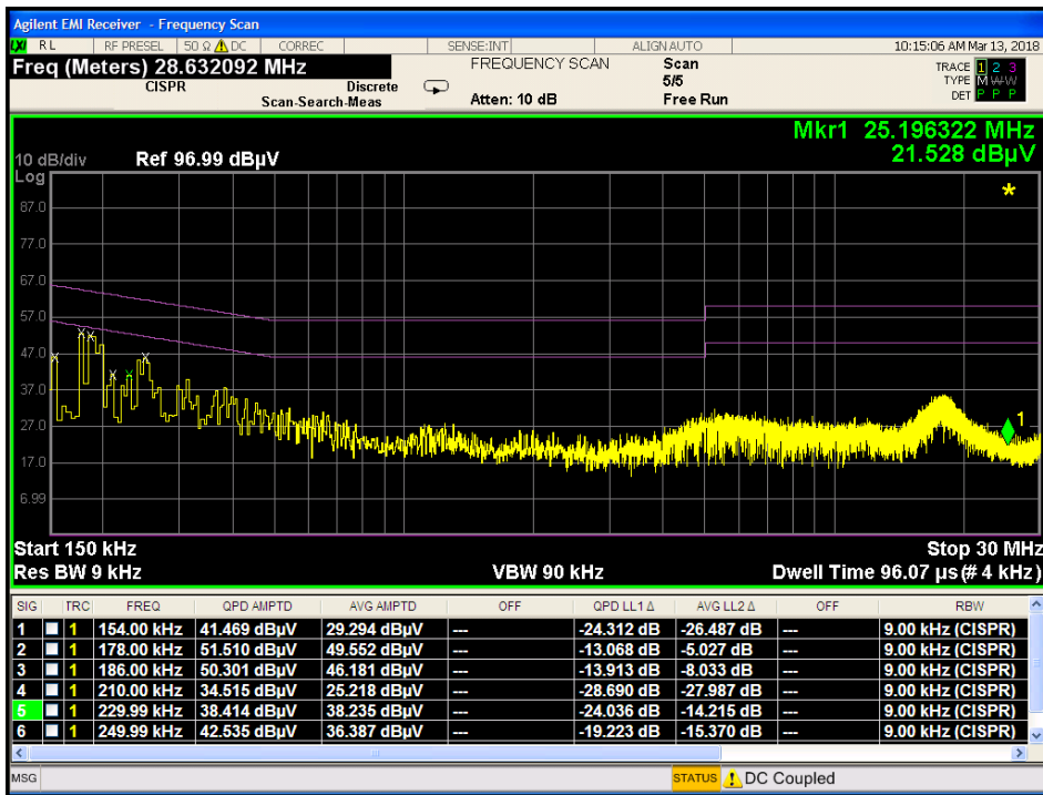
Plot 7-42. Line Conducted Plot and Data with 802.11b (L1)
