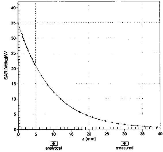
f = 2600 MHz, WGLS R22 (M_convF)
