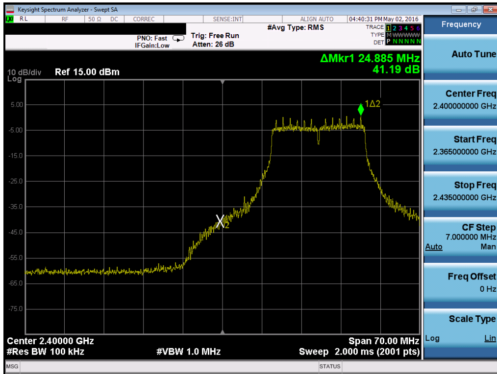
Plot 7-22. Band Edge Plot (802.11g - Ch. 2)
