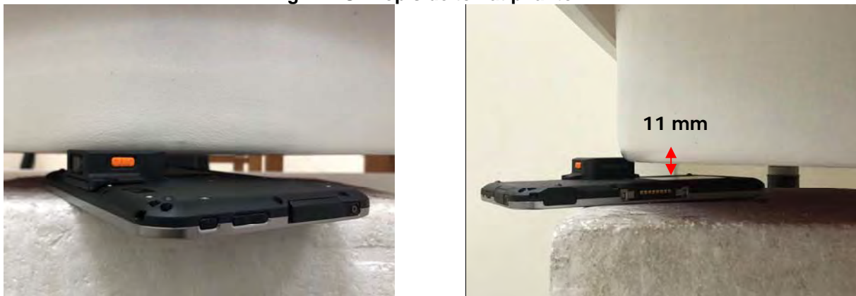
Fig.25 EUT Back side (Landscape scanner) to flat phantom
