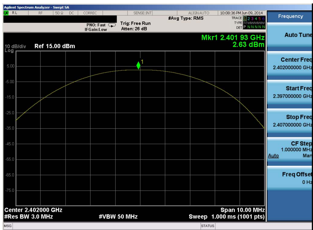
Plot 6-4. Peak Power Plot (Bluetooth (LE) – Ch. 0)
