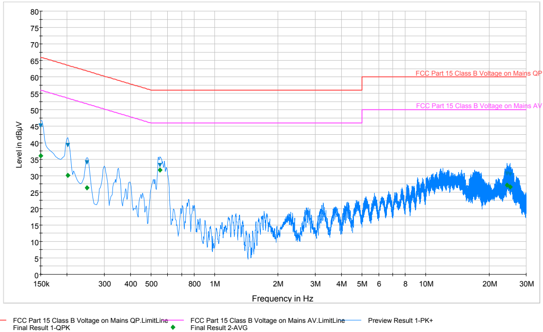
Plot 6-40. Line Conducted Plot with 802.11b (N)
