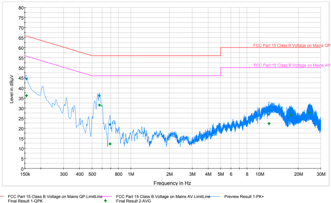
Plot 6-39. Line Conducted Plot with 802.11b (L1)
