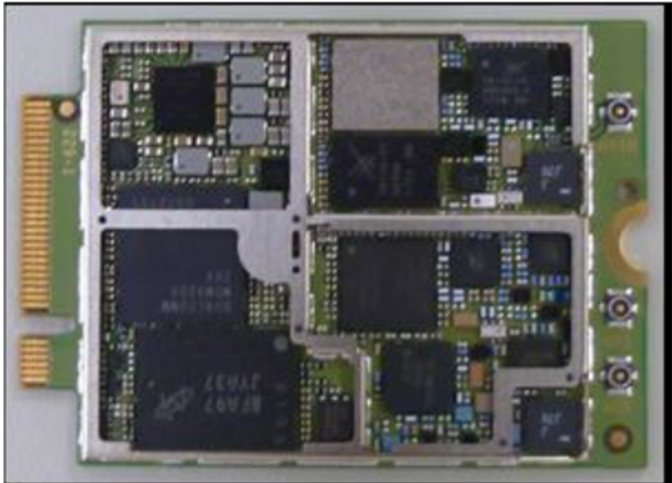
Shield removed
