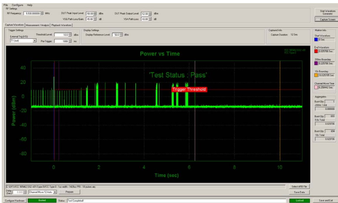
Figure 5-8. Band 2C Move Time and Aggregate Time
