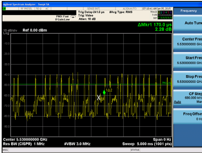
Figure 5-5. Band 2C Pulse Width
