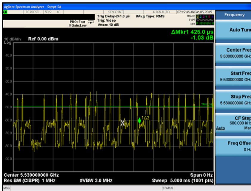
Figure 5-6. Band 2C Period
