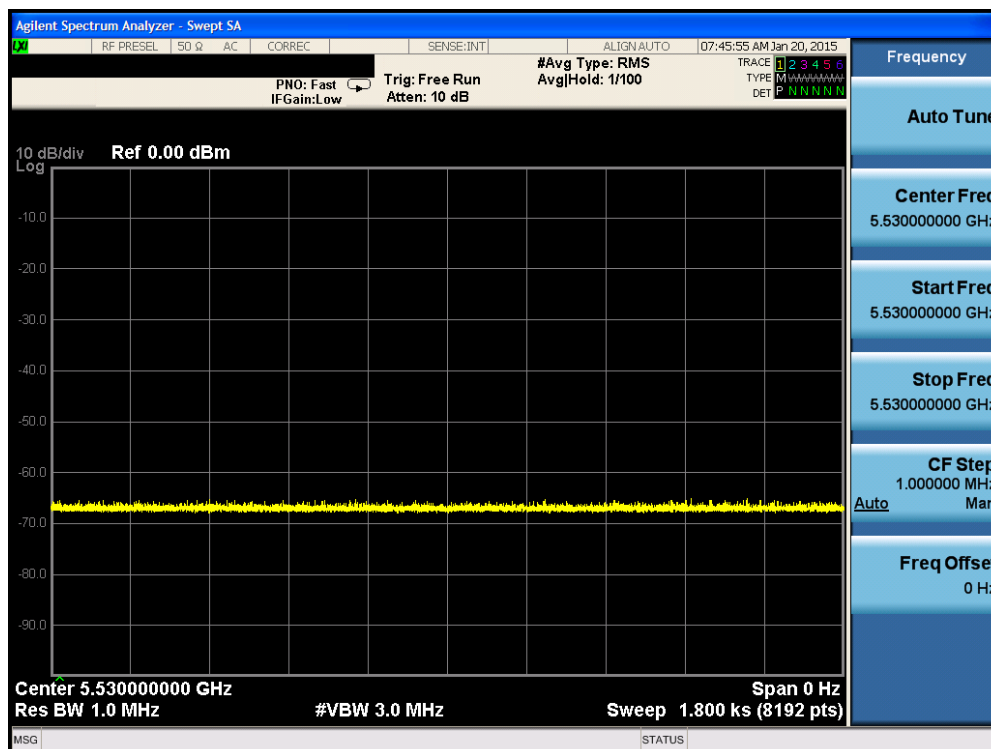
Figure 5-10. Band 2C Non-occupancy Period - Monitoring live spectrum - Elapse time 30 minutes
