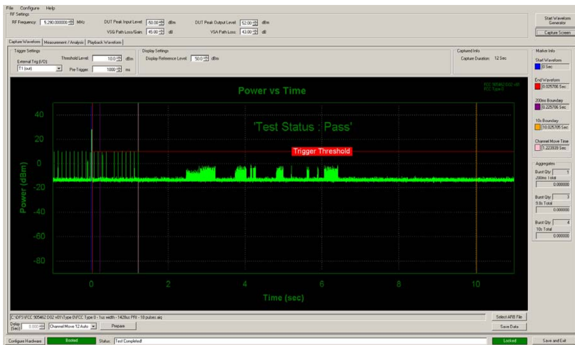
Figure 5-7. Band 2A Move Time and Aggregate Time
