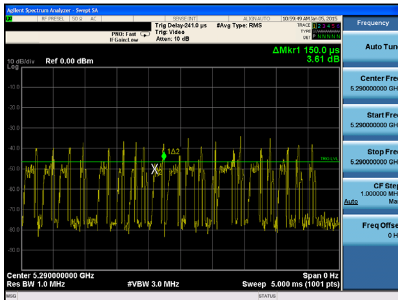
Figure 5-3. Band 2A Pulse Width
