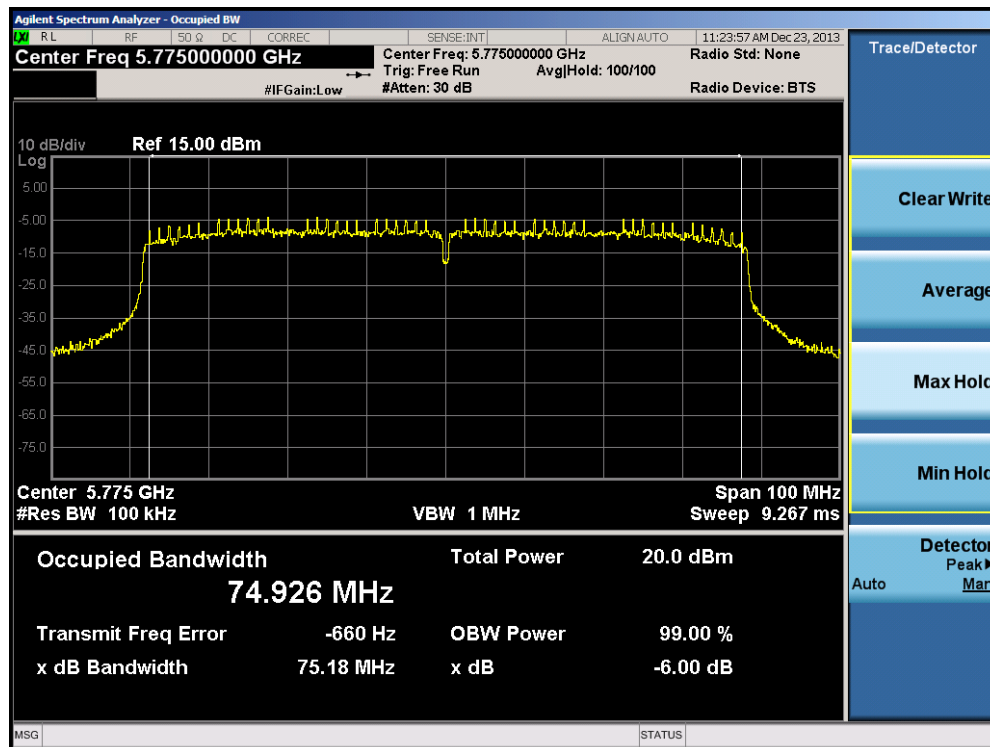
Plot 6-38. 6dB Bandwidth Plot (80MHz BW 802.11ac (UNII Band 3) – Ch. 155)
