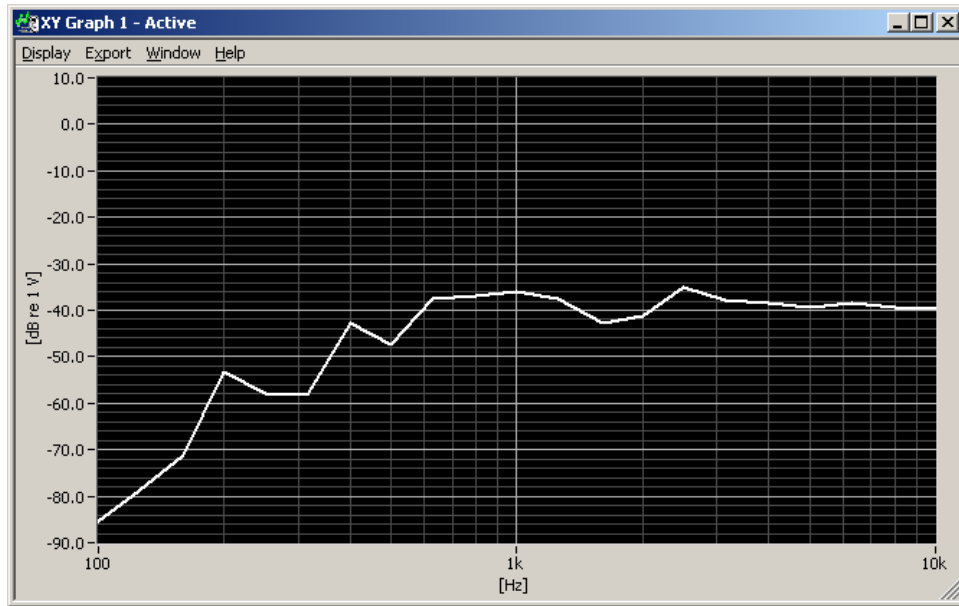
Figure 6-3 Worst-case ABM2 Plot for GSM
