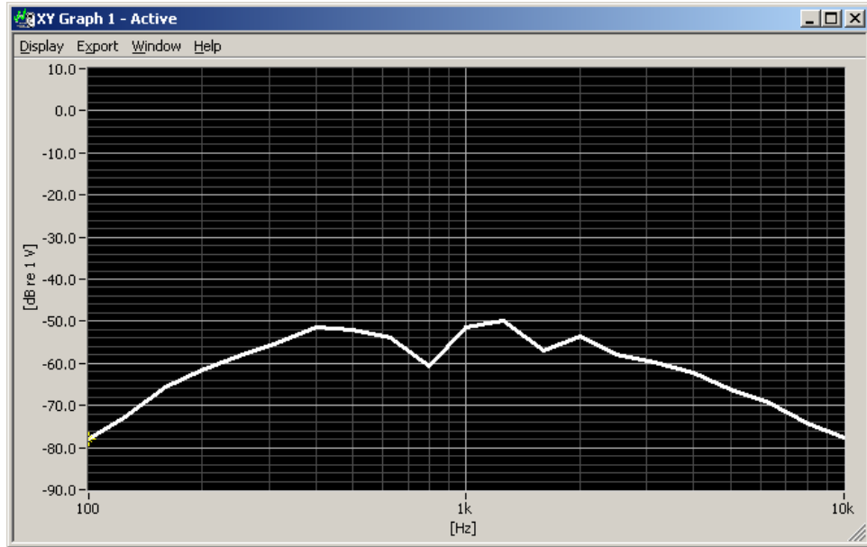
Figure 6-2 Worst-case ABM2 Plot for CDMA
