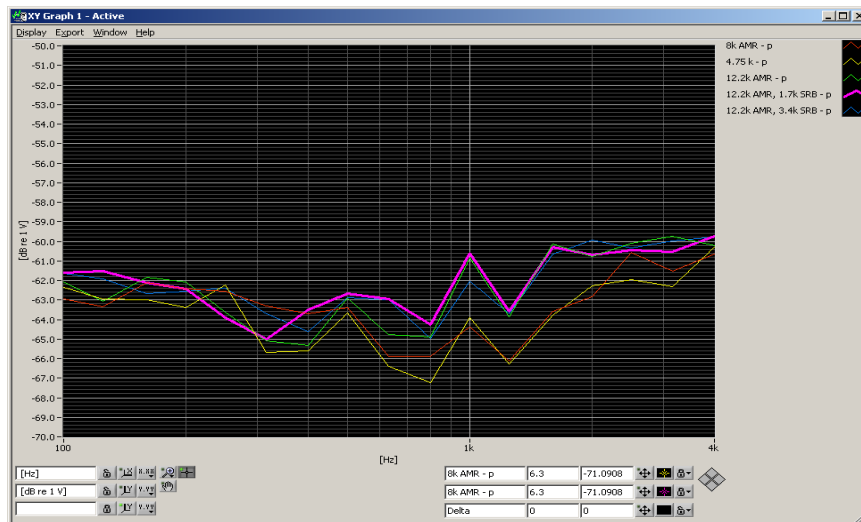
Figure 5-2 UMTS Audio Band Magnetic Noise
