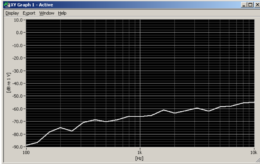
Figure 6-4 Worst-case ABM2 Plot for UMTS
