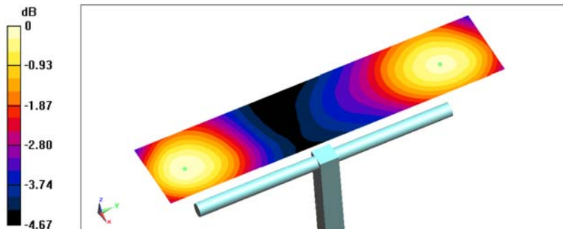
0 dB = 93.75 V/m = 39.44 dBV/m
