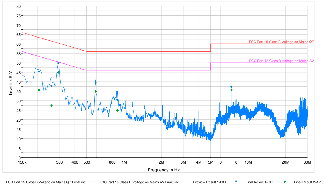
Plot 6-73. Line Conducted Plot with 802.11a (N)
