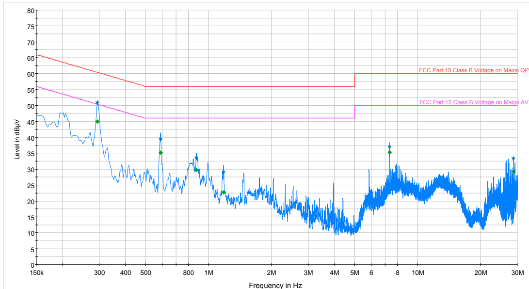
Plot 6-72. Line Conducted Plot with 802.11a (L1)
