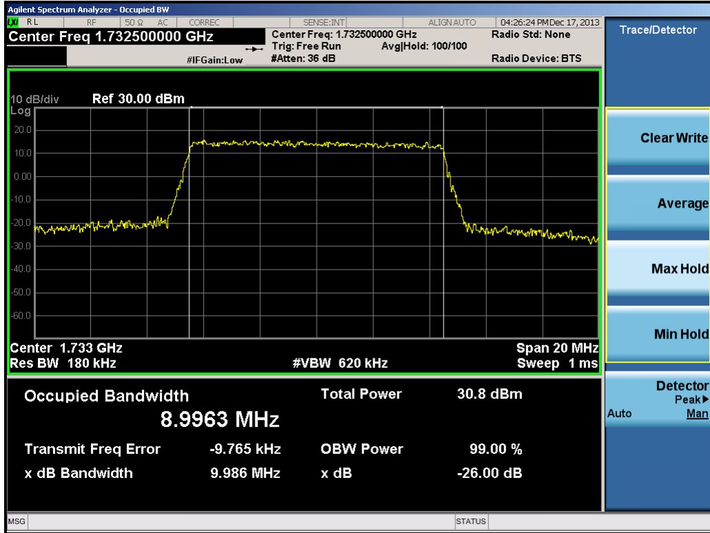
Plot 9-14. Occupied Bandwidth Plot (10.0MHz QPSK – RB Size 50)
