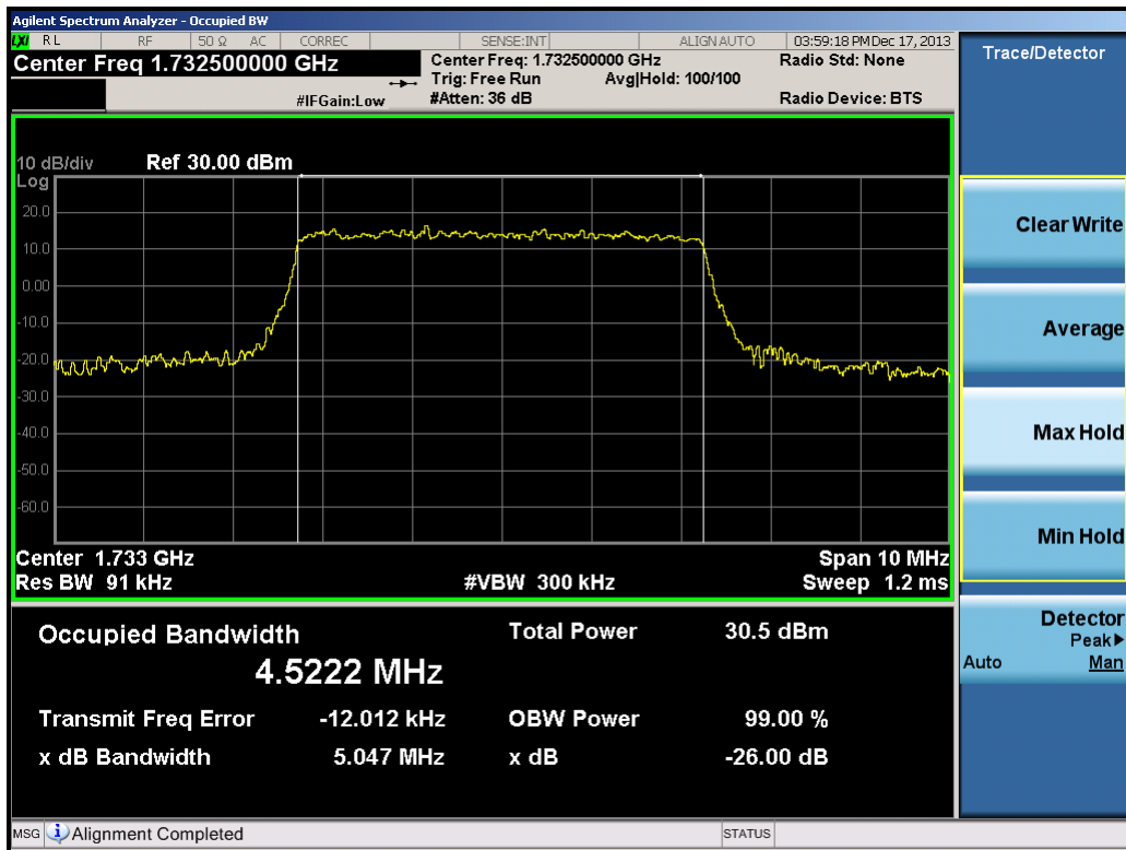
Plot 9-3. Occupied Bandwidth Plot (5.0MHz 16-QAM – RB Size 25)
