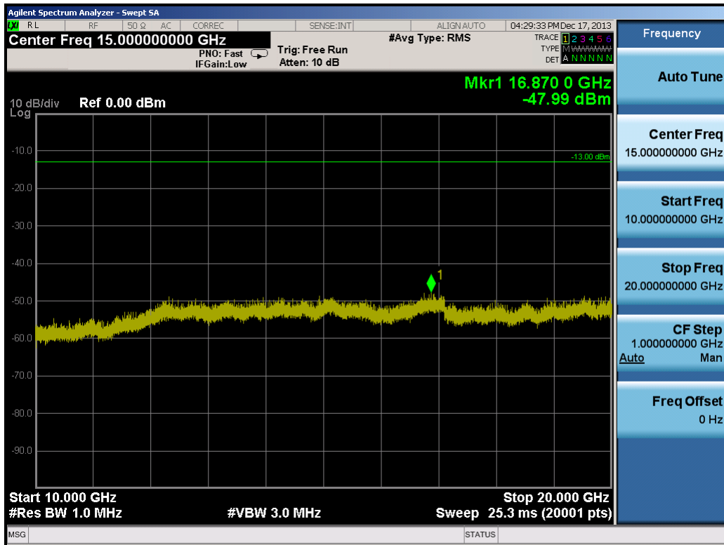
Plot 9-17. Conducted Spurious Plot (10.0MHz QPSK – RB Size 1, RB Offset 0 – Low Channel)
