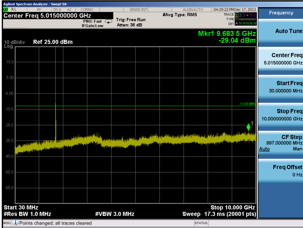
Plot 9-16. Conducted Spurious Plot (10.0MHz QPSK – RB Size 1, RB Offset 0– Low Channel)
