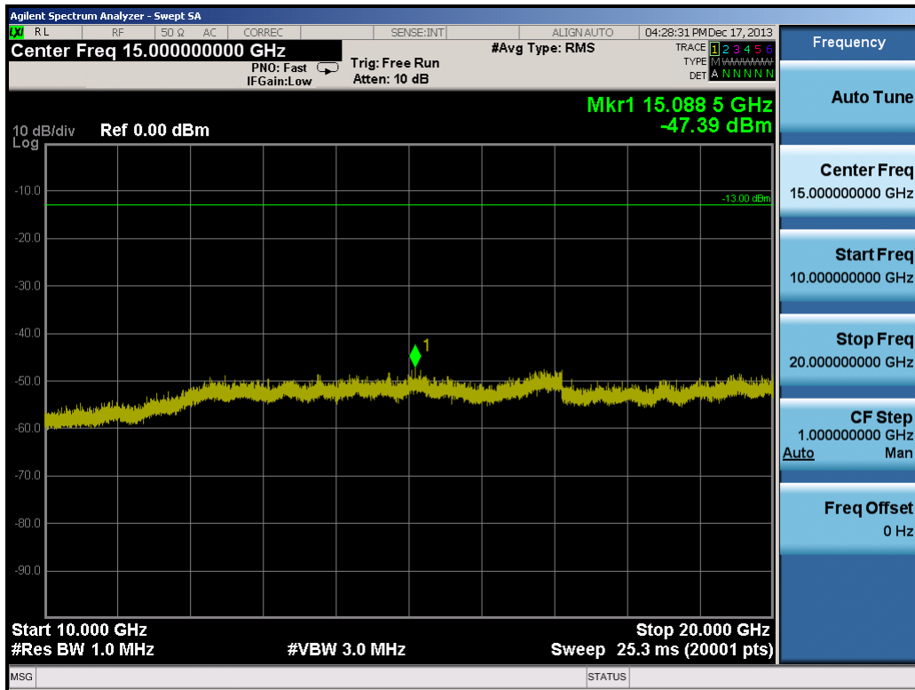
Plot 9-19. Conducted Spurious Plot (10.0MHz QPSK – RB Size 1, RB Offset 0 – Mid Channel)
