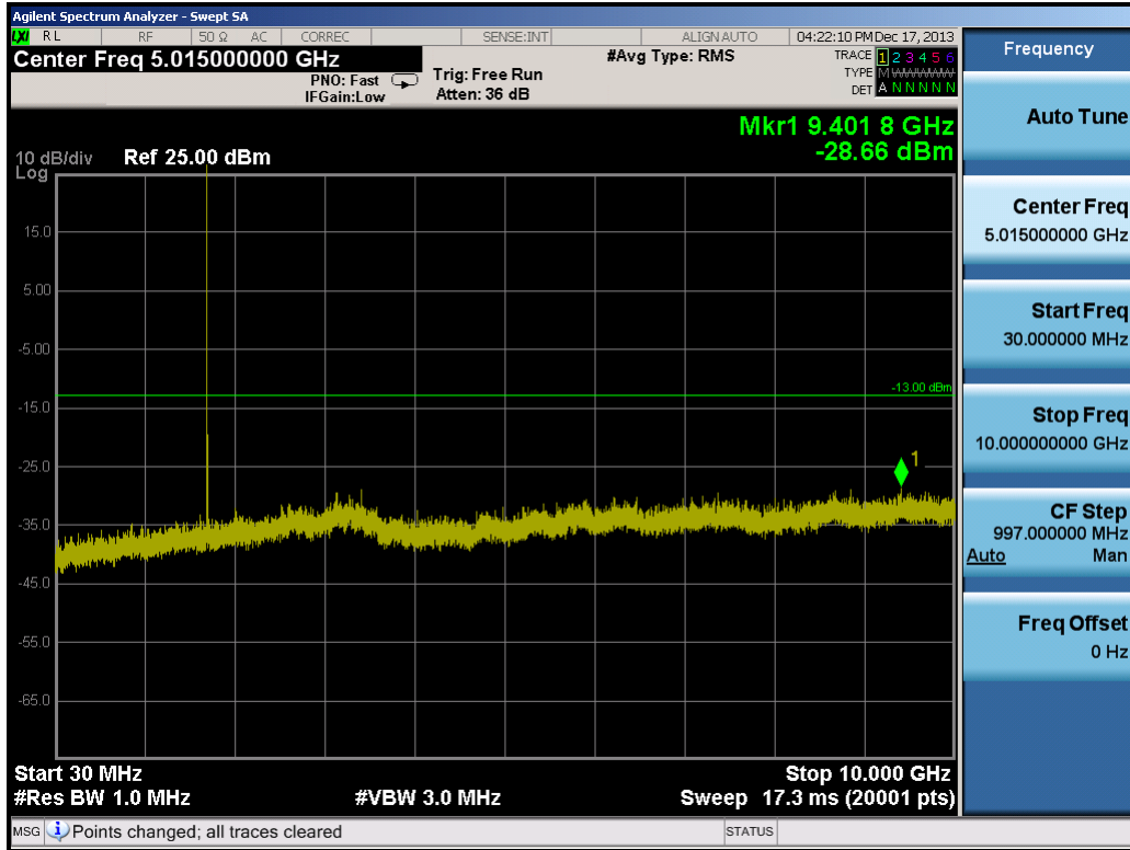
Plot 9-4. Conducted Spurious Plot (5.0MHz QPSK – RB Size 1, RB Offset 0 – Low Channel)
