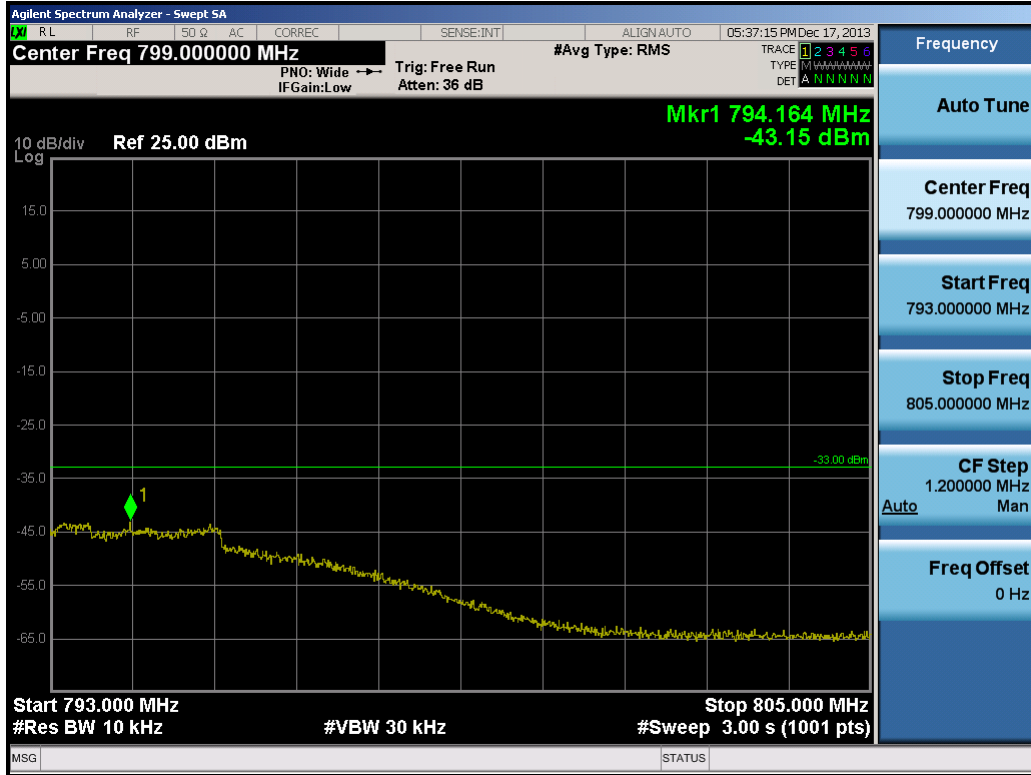
Plot 8-8. Upper Emission Mask Plot (10.0MHz QPSK – RB Size 50)
