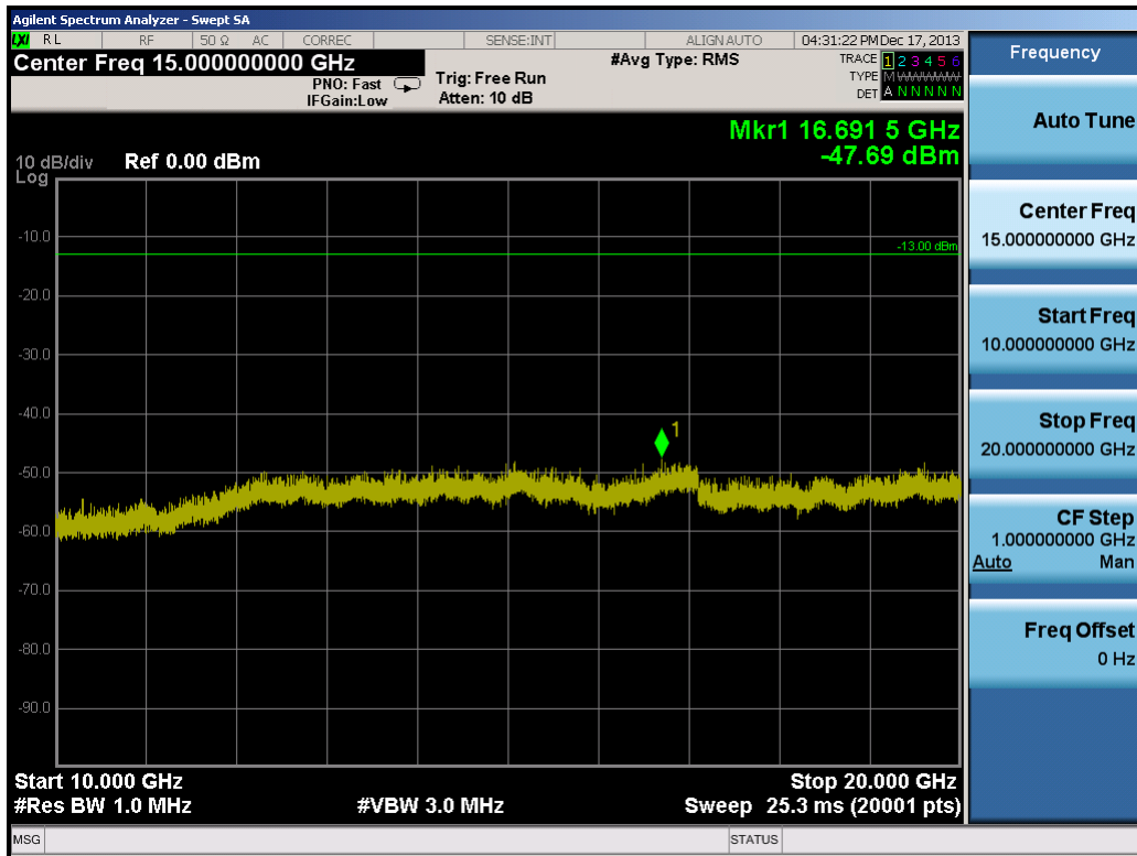
Plot 9-21. Conducted Spurious Plot (10.0MHz QPSK – RB Size 1, RB Offset 0 – High Channel)
