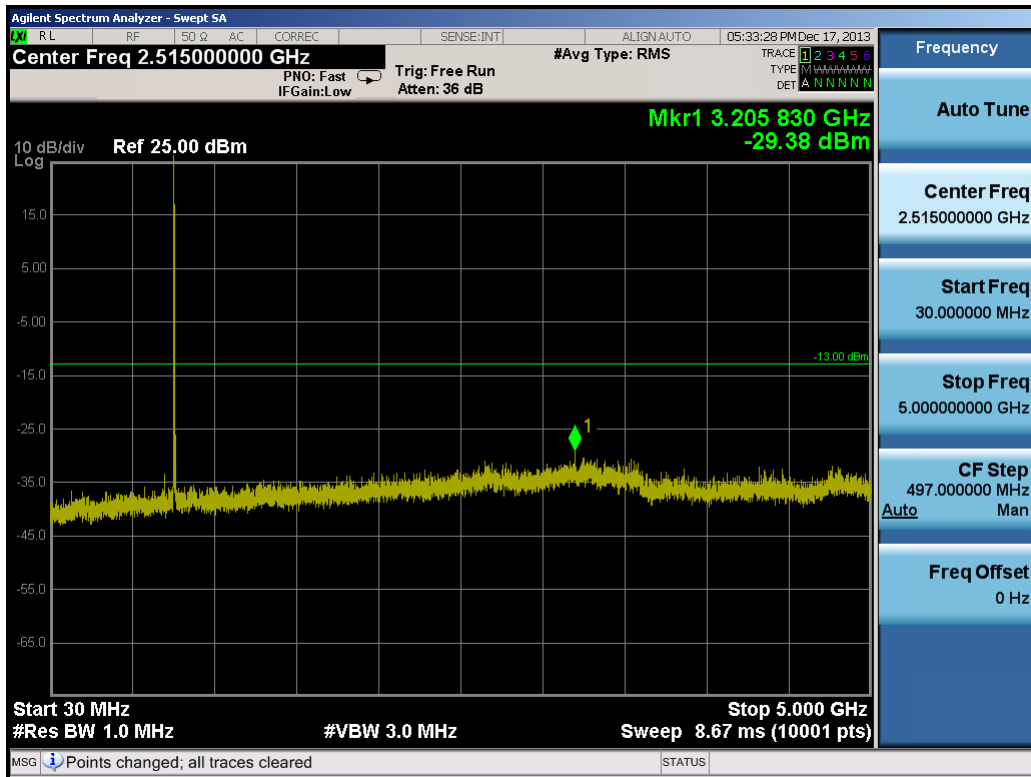
Plot 8-5. Conducted Spurious Plot (10.0MHz QPSK – RB Size 1, RB Offset 0)
