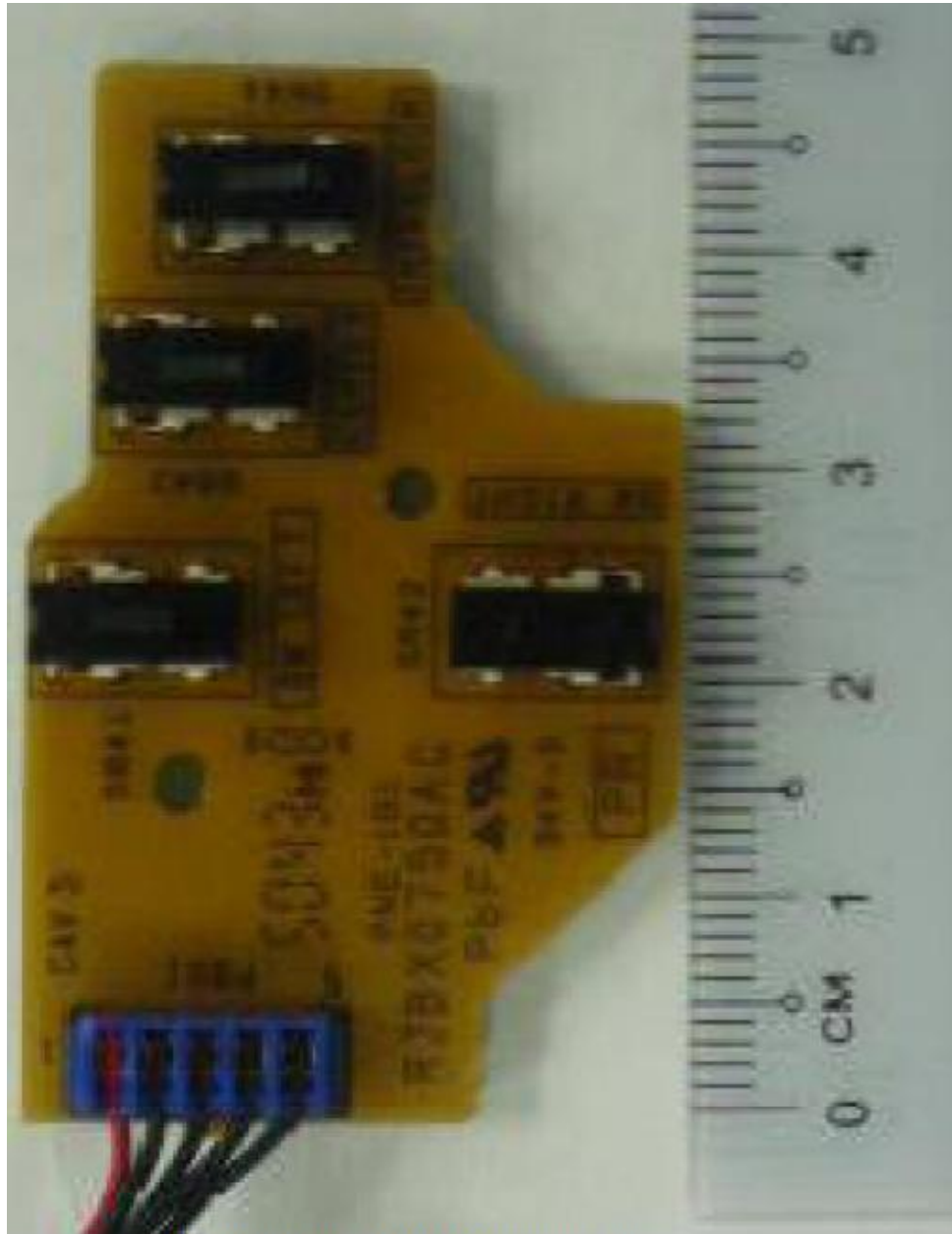
POS Switch Board PCB Component Side
