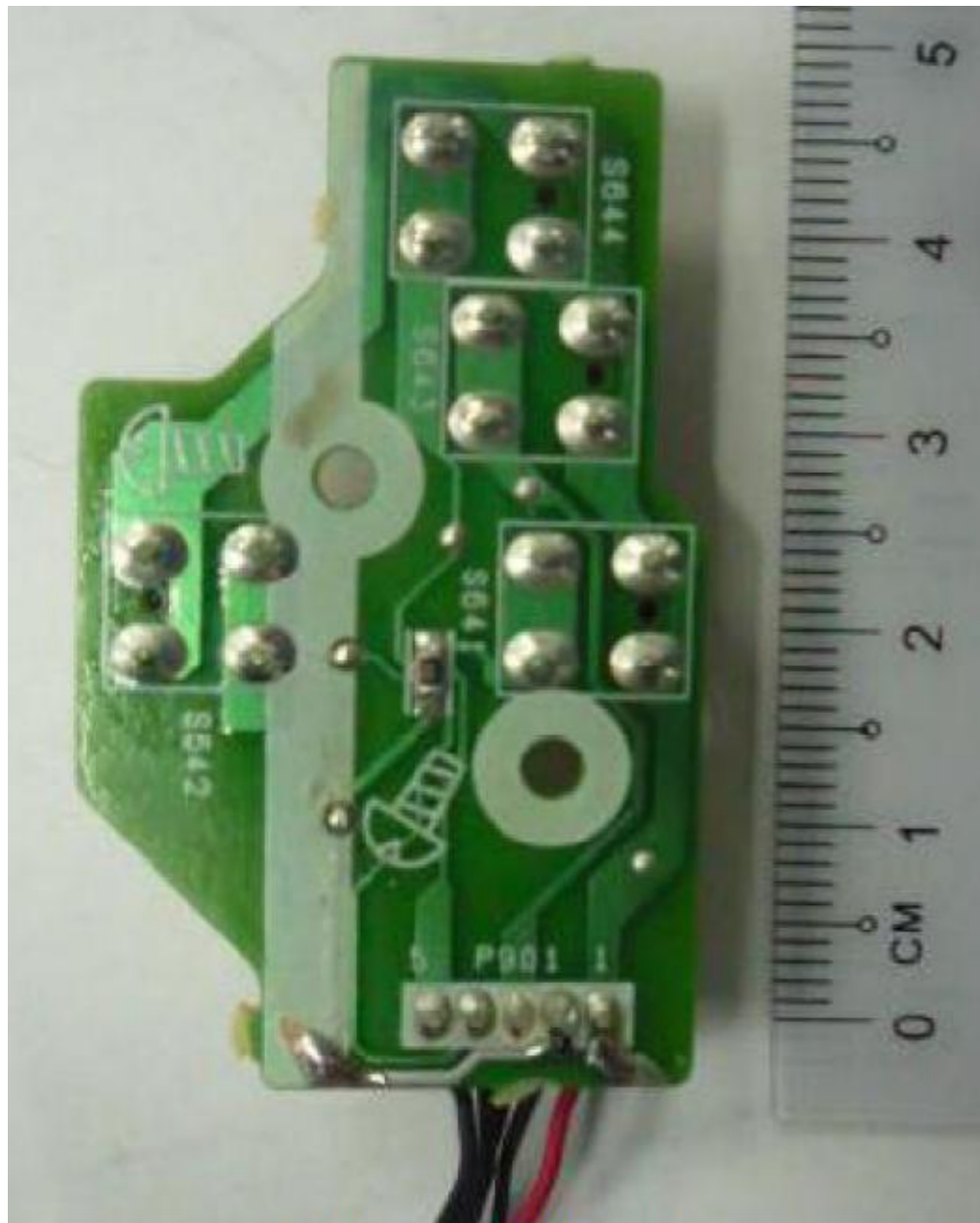
POS Switch Board PCB Trace Side
