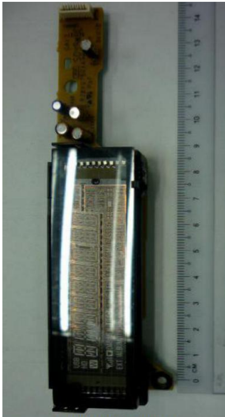
FL Board PCB Component Side
