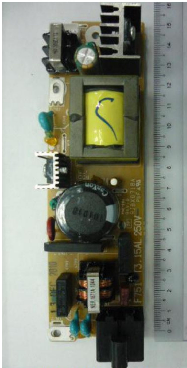
SMPS Board PCB Component Side
