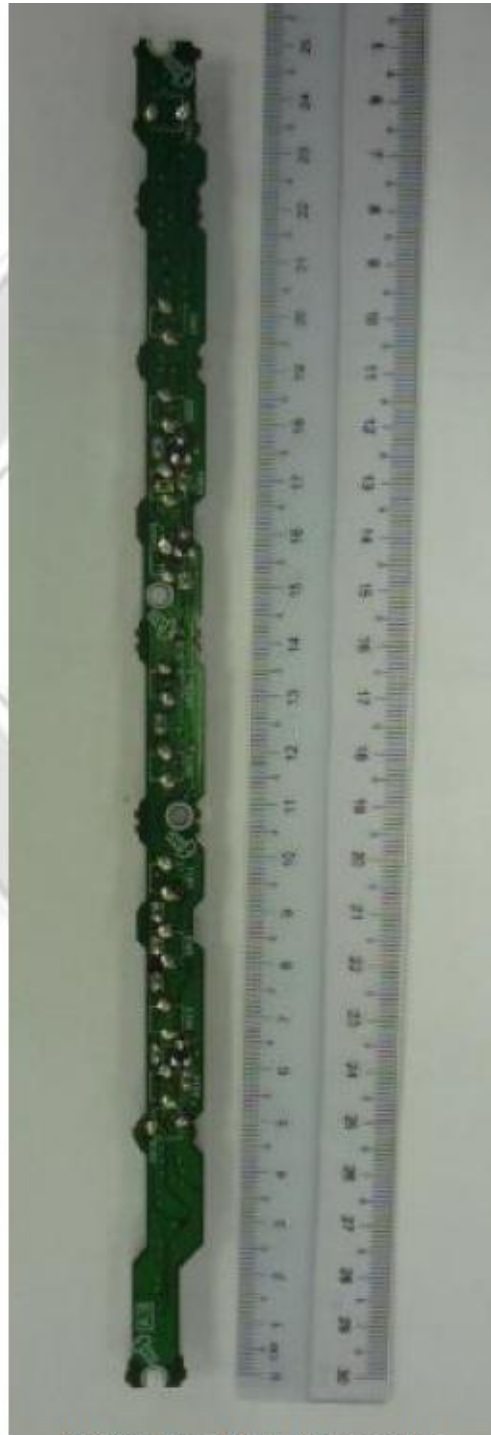
Button Board PCB Trace Side
