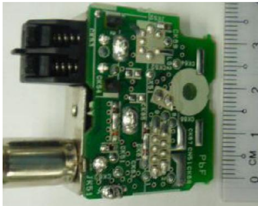
Tuner Board PCB Component Side
