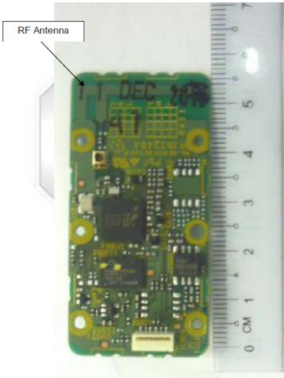
Bluetooth Board PCB Component Side
