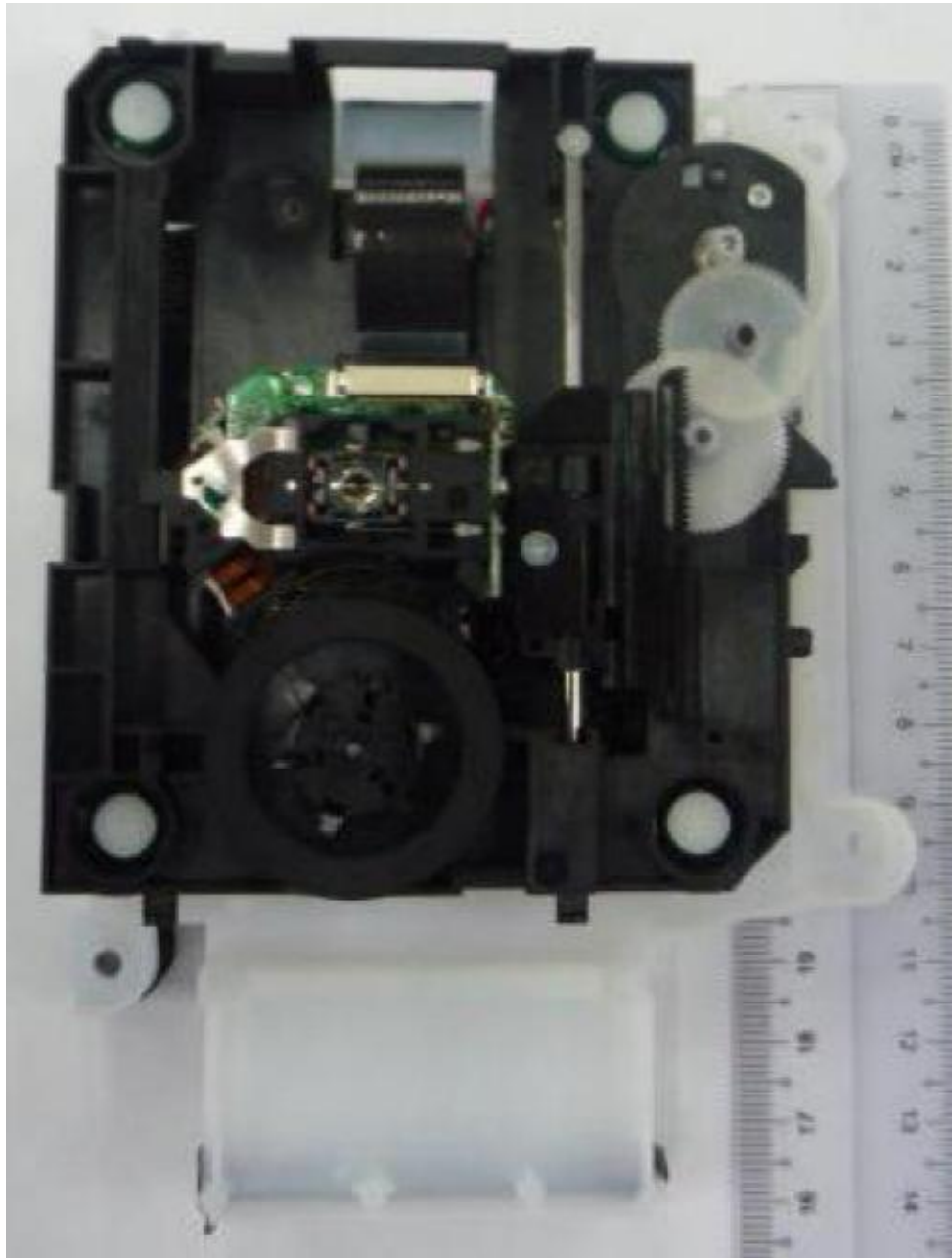
OPU Unit Board PCB Component Side
