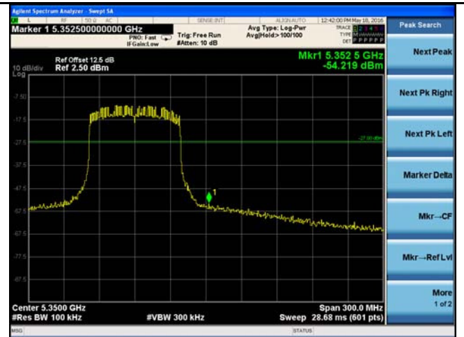
5150-5350MHz Band Edge - High CH 5290
