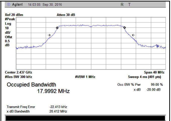
802.11n20 20dB Bandwidth - Mid CH 2437
