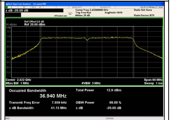
802.11n40 20dB Bandwidth - Low CH 2422
