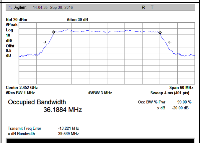
802.11n40 20dB Bandwidth - High CH 2452
