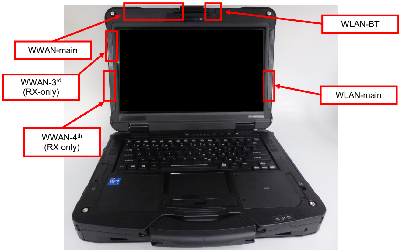
Front view
