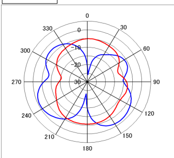
824MHz Red:Vertical
