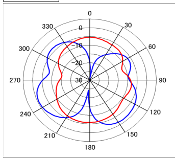
814MHz Red:Vertical
