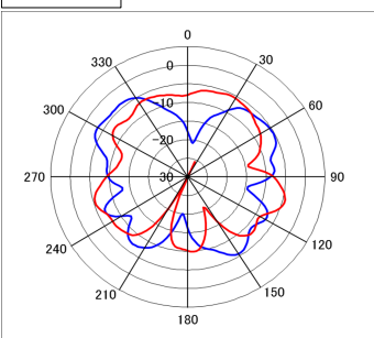
2690MHz Red:Vertical
