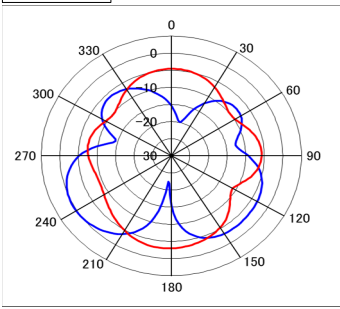
716MHz Red:Vertical
