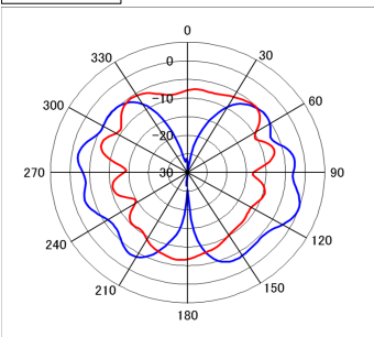
1915MHz Red:Vertical
