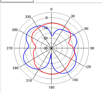
849MHz Red:Vertical
