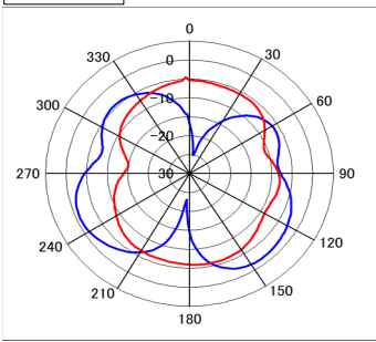
798MHz Red:Vertical
