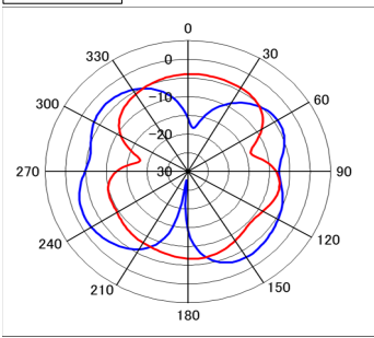
787MHz Red:Vertical
