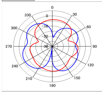
777MHz Red:Vertical
