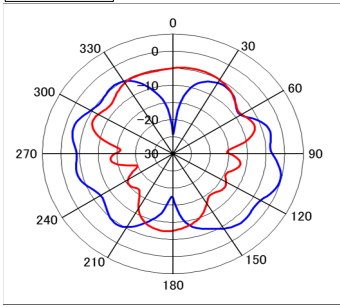
1780MHz Red:Vertical
