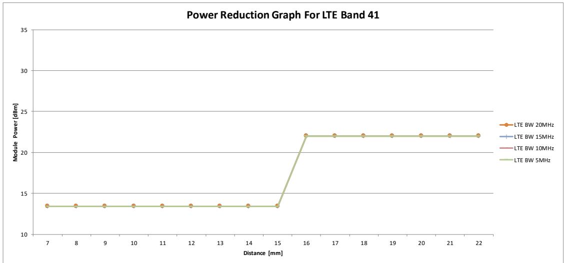
LTE B41
