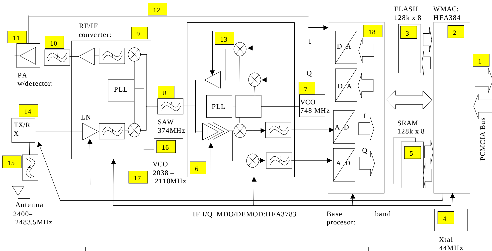
Block Diagram – Panasonic Wireless LAN radio module (WT M 1)
