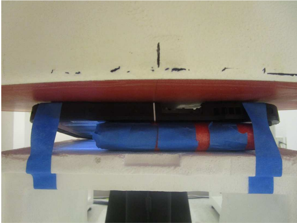
Photograph 10: Body, Rear Tilt (Edge1 side), 0 mm (side view)
