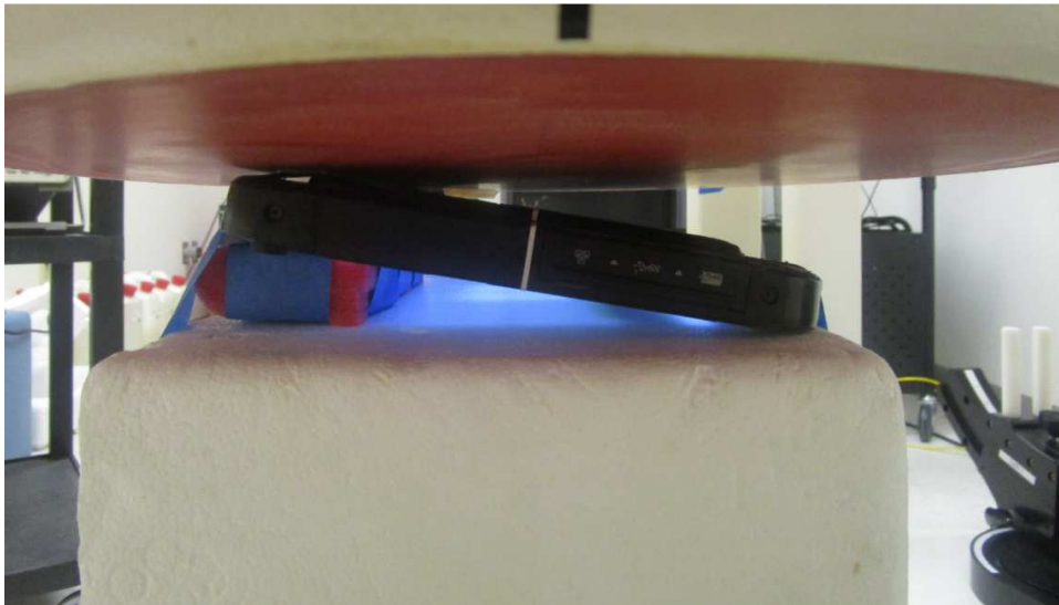
Photograph 10: Body, Rear Tilt (Edge1 side), 0 mm (side view)
