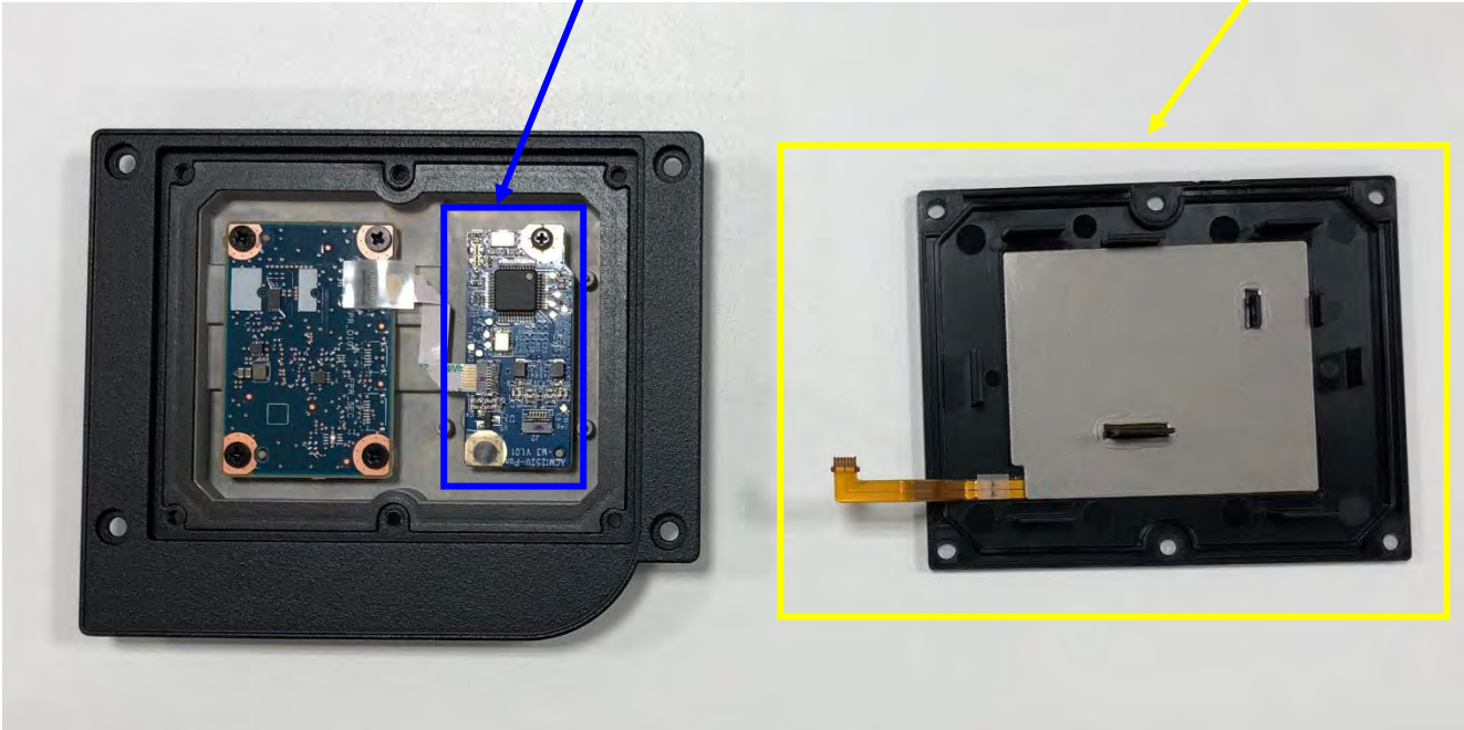
HF-RFID antenna
