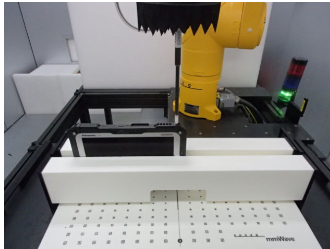
Module #1 (Edge 1)
