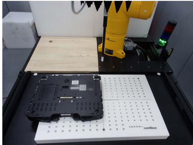
Module #1 (Bottom)
