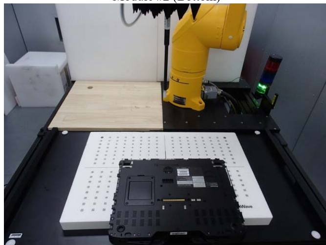
Module #2 (Bottom)
