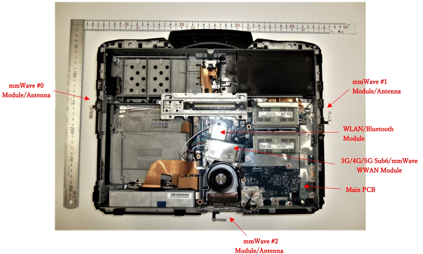
Internal view - Bottom
