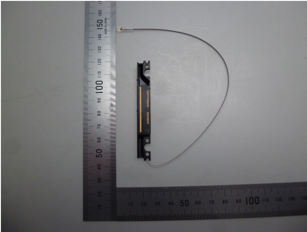
WWAN-4th TX/RX Antenna – Front
