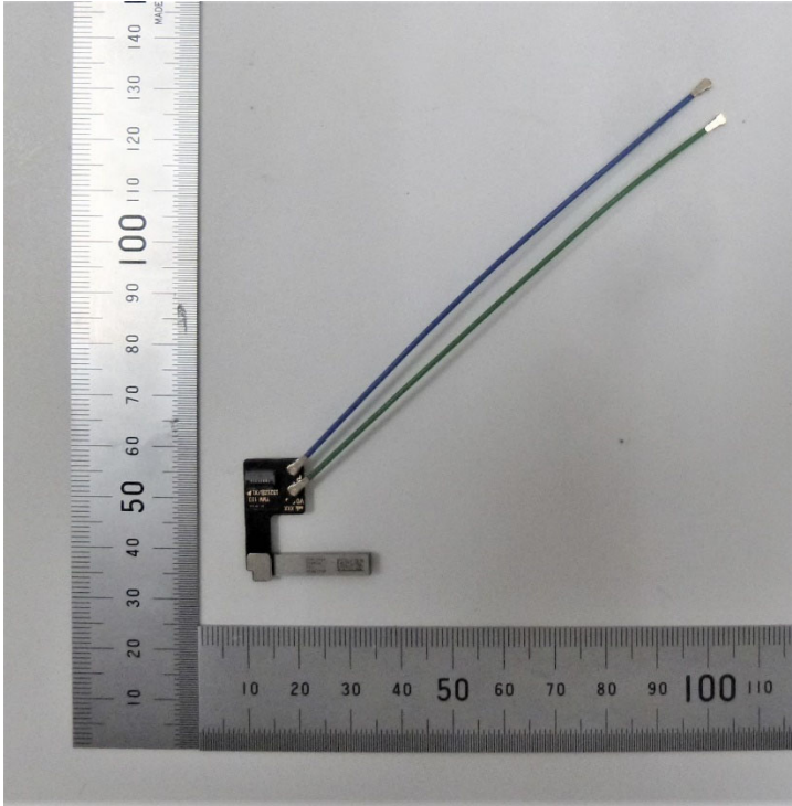
mmWave #2 Module/Antenna - Back
