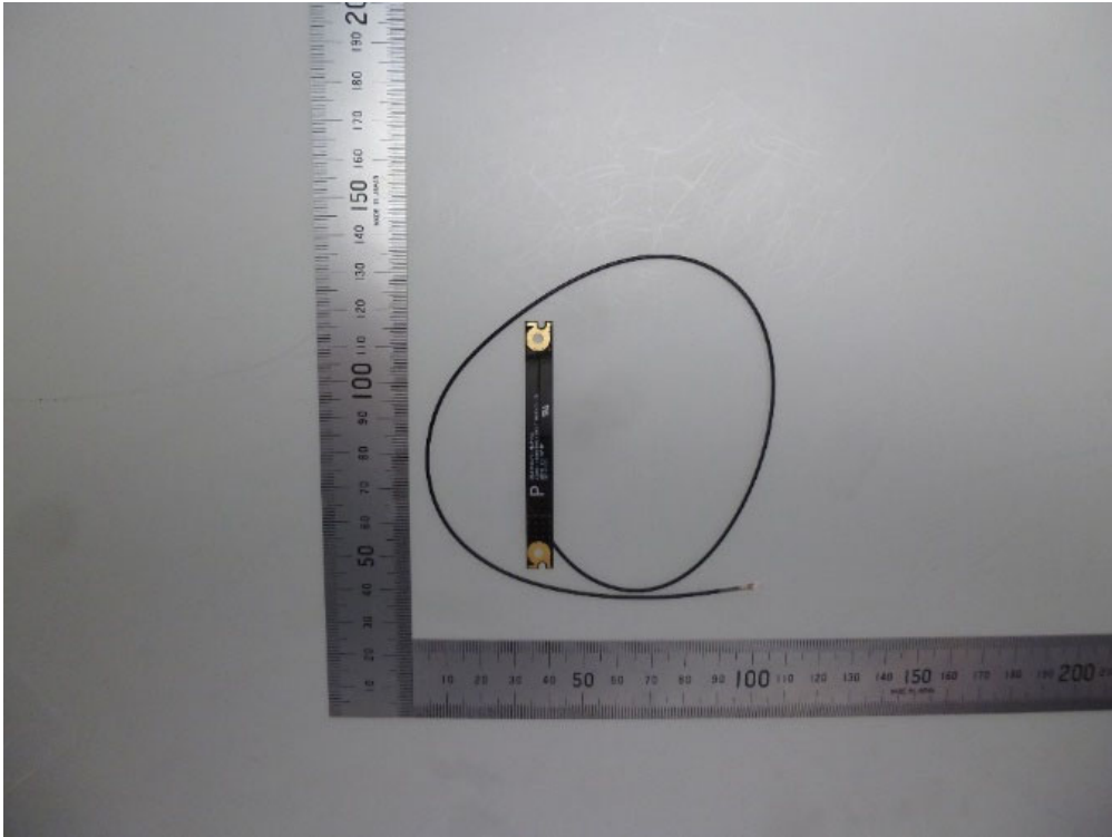
WLAN-main TX/RX Antenna - Front
