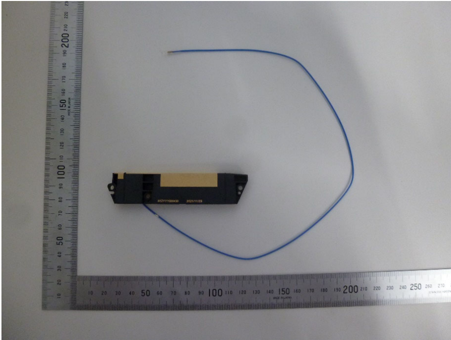
WWAN-main TX/RX Antenna - Front
