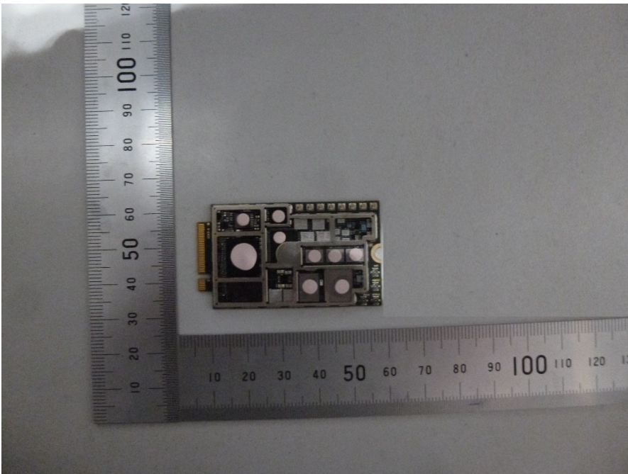
3G/4G/5G Sub6/mmWave WWAN Module without shield cover - Front
