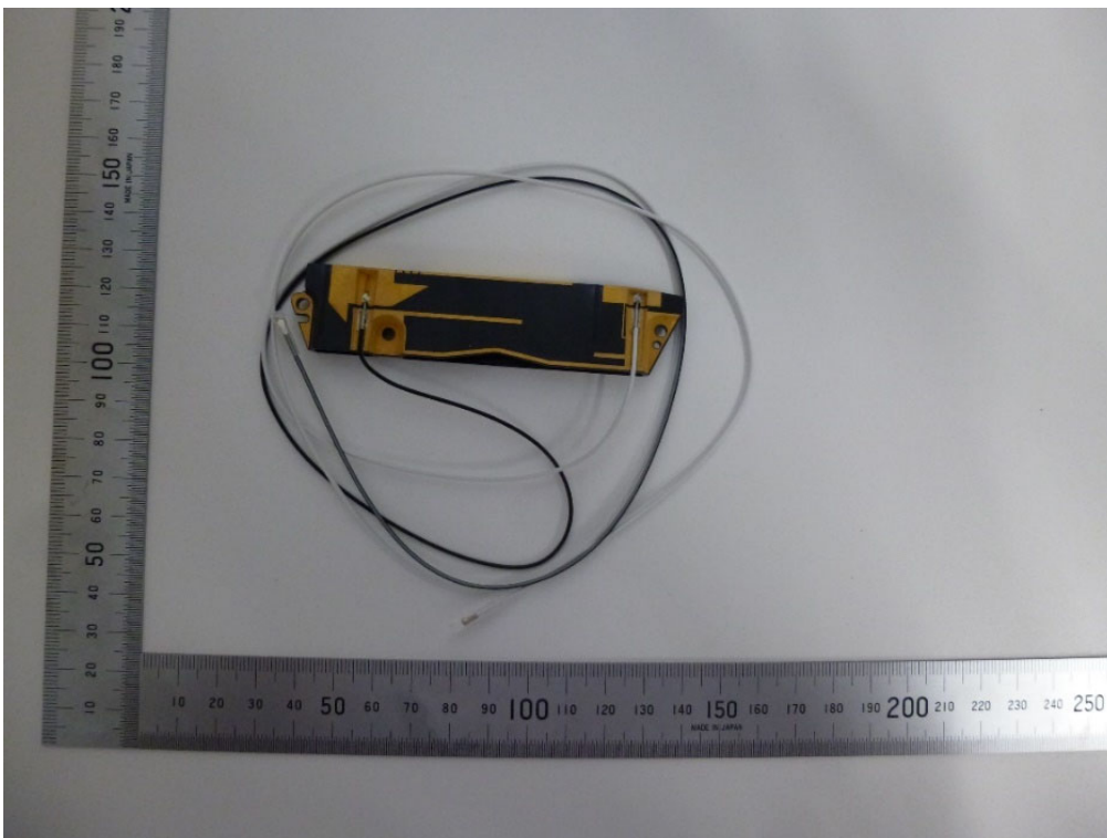
WLAN-BT TX/RX Antenna & WWAN-aux RX Antenna - Back
