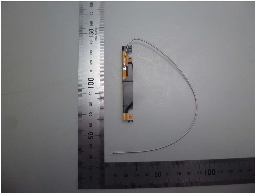
WWAN-4th TX/RX Antenna – Back
