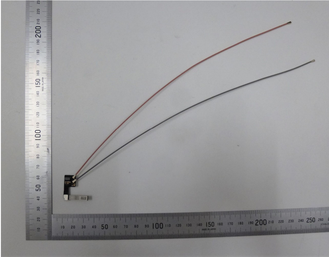
mmWave #0 Module/Antenna – Back
