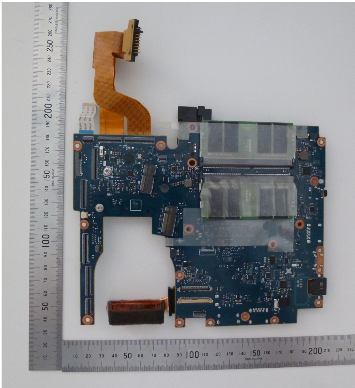
Main PCB – Back
