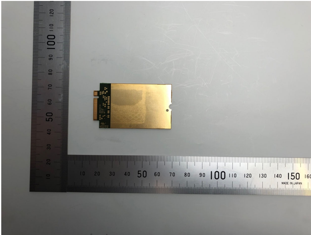
3G/4G/5G Sub6 mmWave WWAN Module - Back
