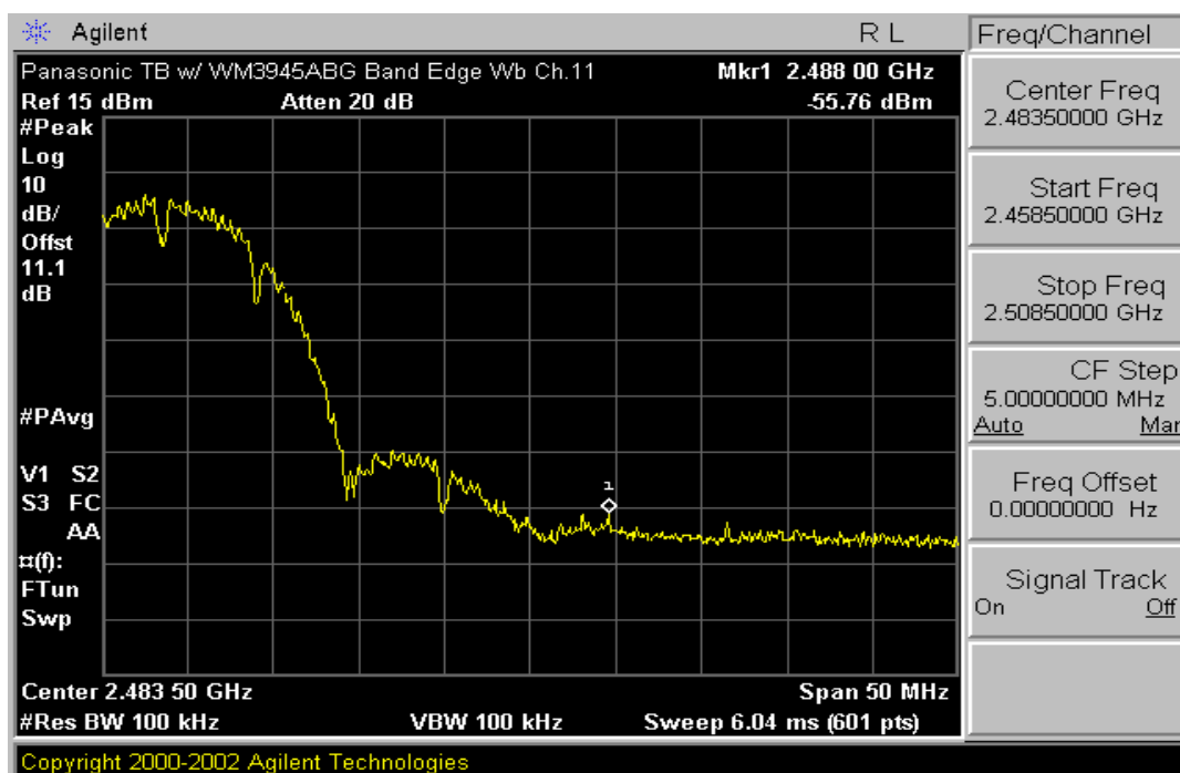
Plot 6-20. Band Edge Plot (802.11b – Ch. 11)
