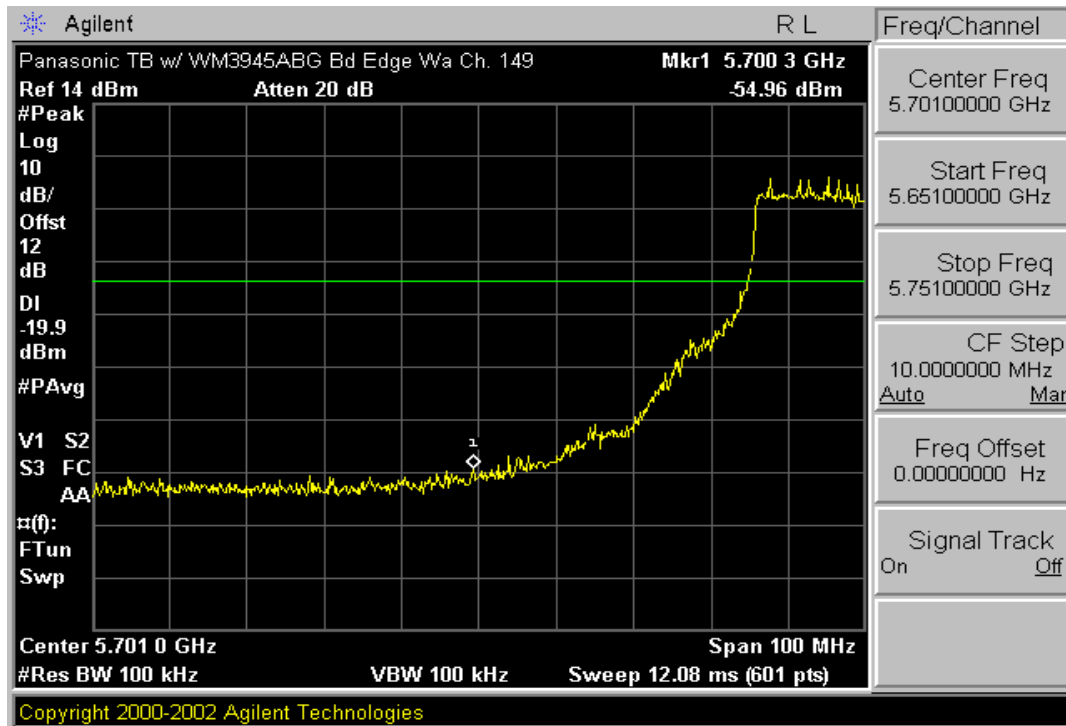
Plot 6-23. Band Edge Plot (802.11a – Ch. 149)
