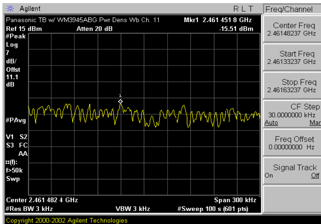
Plot 6-12. Power Spectral Density Plot (802.11b – Ch. 11)
