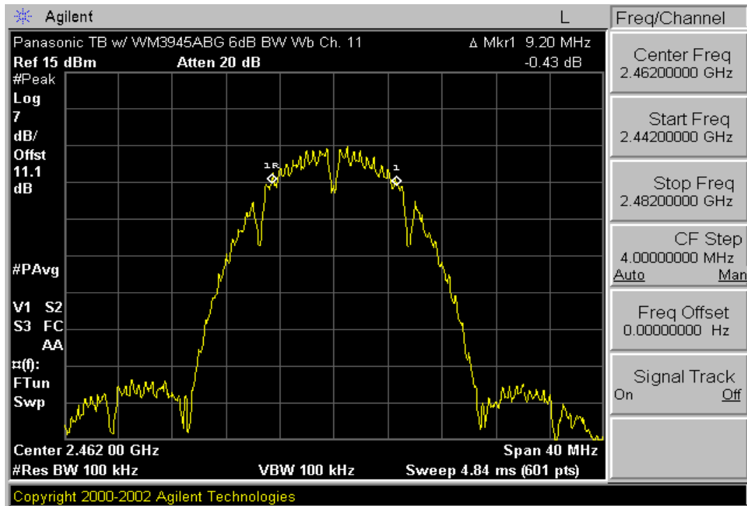
Plot 6-3. 6dB Bandwidth Plot (802.11b – Ch. 11)
