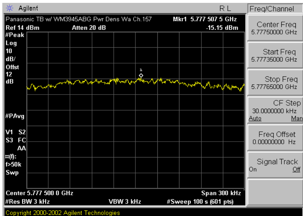
Plot 6-17. Power Spectral Density Plot (802.11a – Ch. 157)
