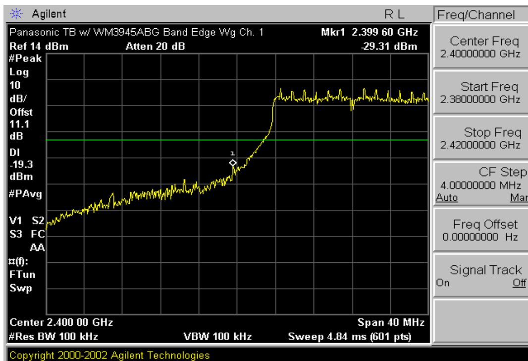
Plot 6-21. Band Edge Plot (802.11g– Ch. 1)
