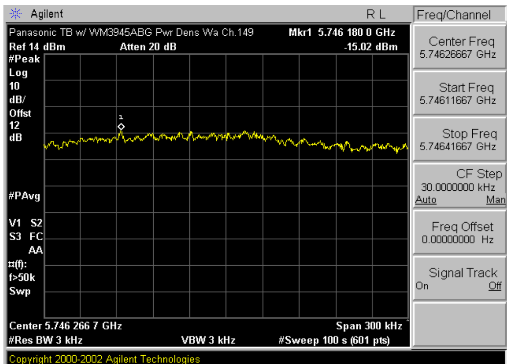
Plot 6-16. Power Spectral Density Plot (802.11a – Ch. 149)
