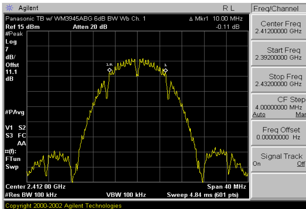
Plot 6-1. 6dB Bandwidth Plot (802.11b – Ch. 1)
