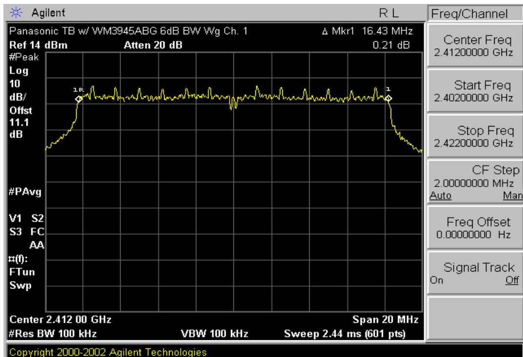
Plot 6-4. 6dB Bandwidth Plot (802.11g – Ch. 1)
