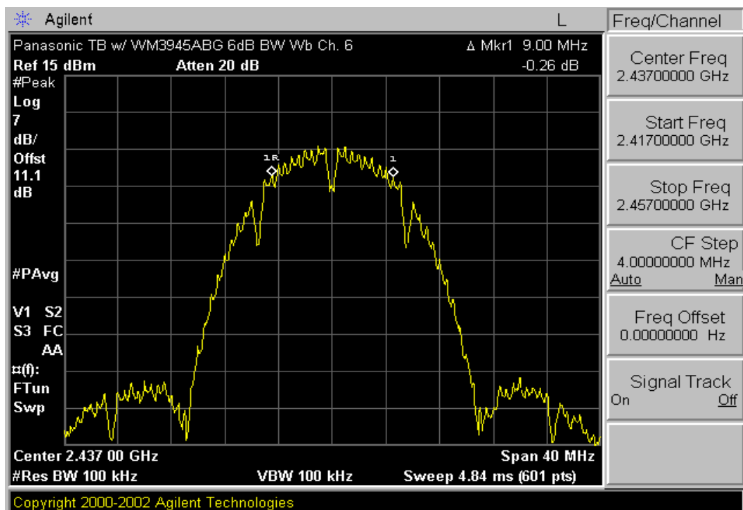
Plot 6-2. 6dB Bandwidth Plot (802.11b – Ch. 6)
