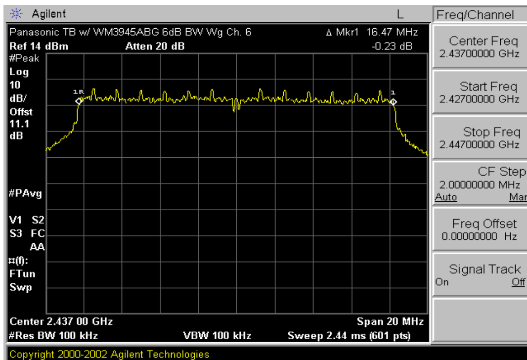
Plot 6-5. 6dB Bandwidth Plot (802.11g – Ch. 6)
