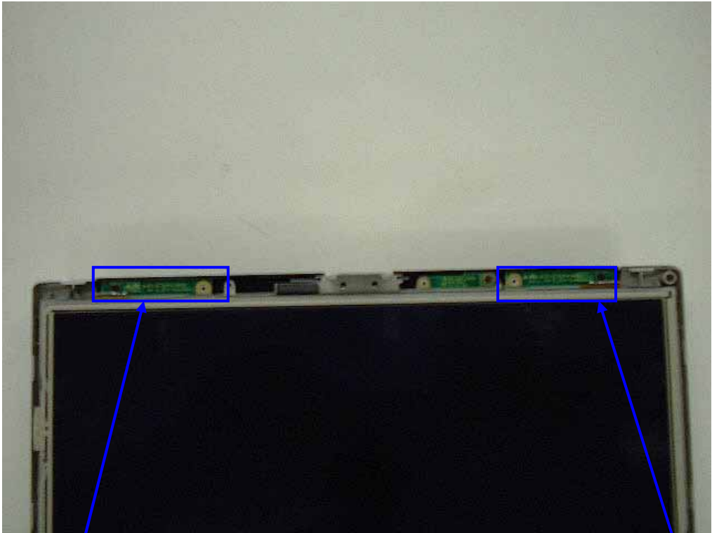
Aux TX/RX WLAN Antenna
