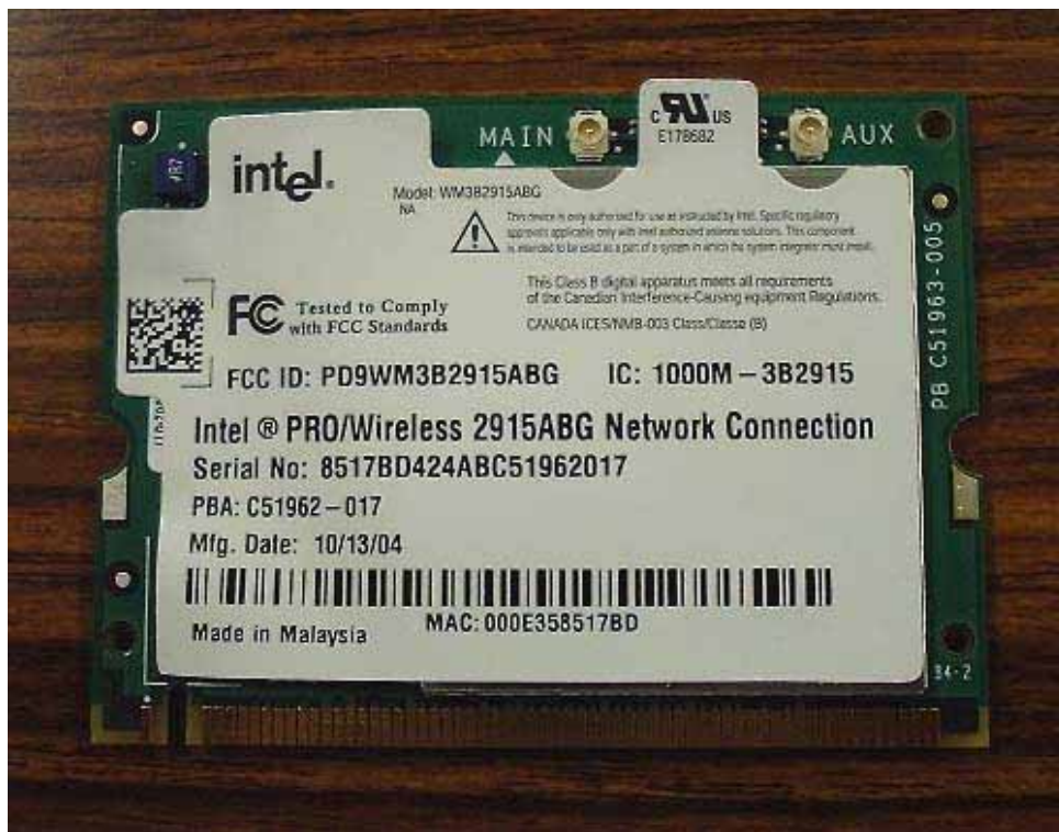
WLAN Top View
