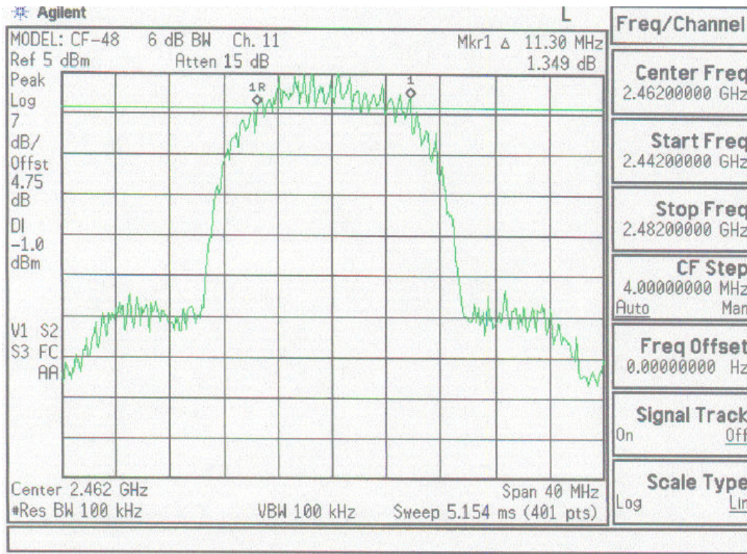
Plot A-3. 6dB Bandwidth Plot – Ch.11
