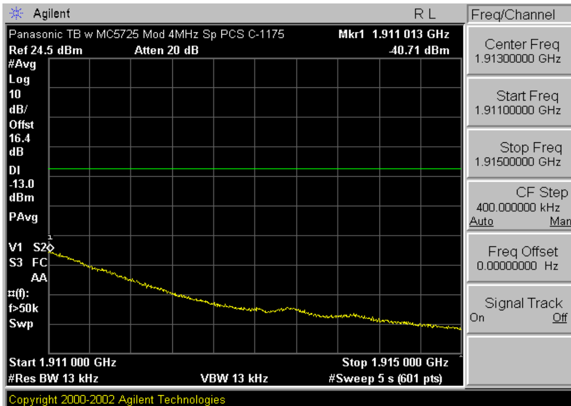
Plot A-24. 4MHz Span Plot (PCS CDMA EvDO Mode – Ch. 1175)
