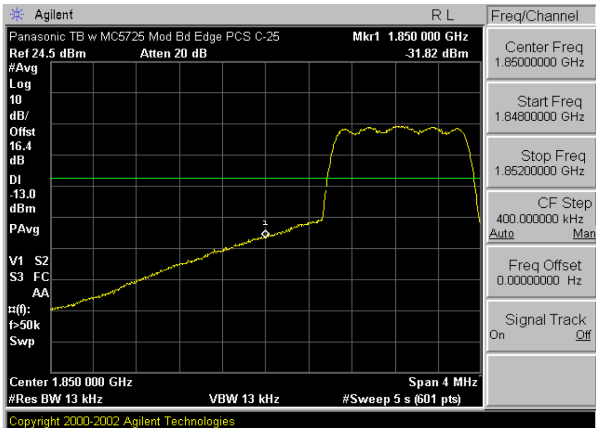
Plot A-15. Band Edge Plot (PCS CDMA EvDO Mode – Ch. 25)
