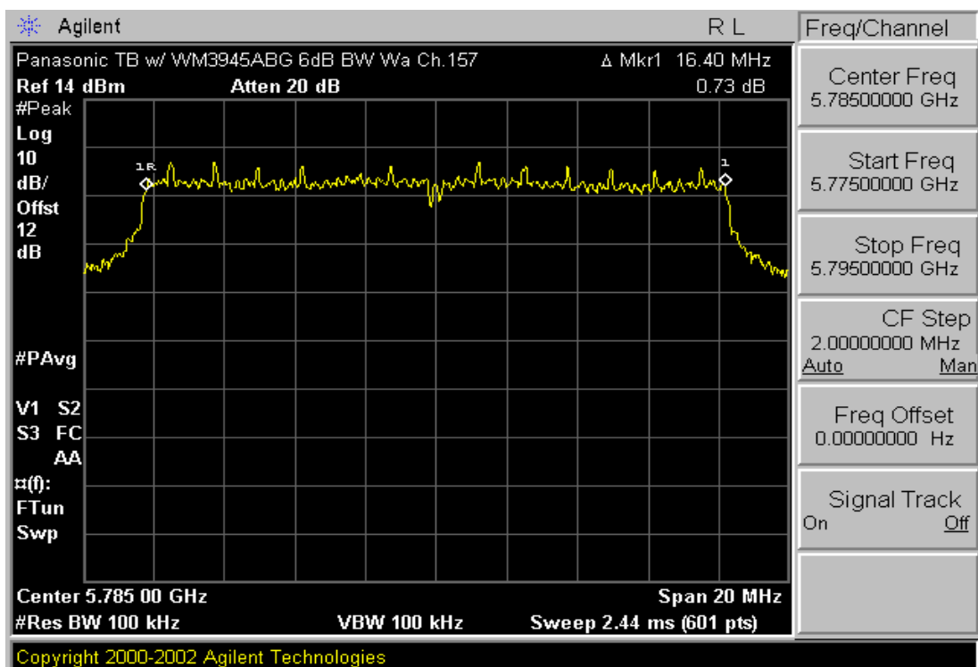
Plot 6-8. 6dB Bandwidth Plot (802.11a – Ch. 157)
