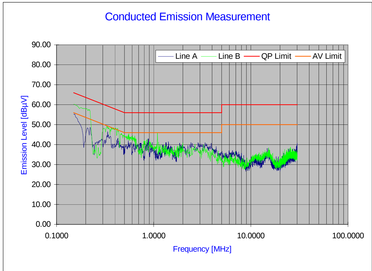
Plot 6-25. Line Conducted Plot with 802.11b
