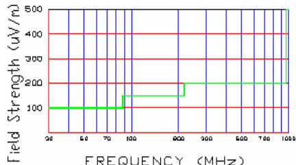
Figure 6-10. Radiated limits at 3 meters.
