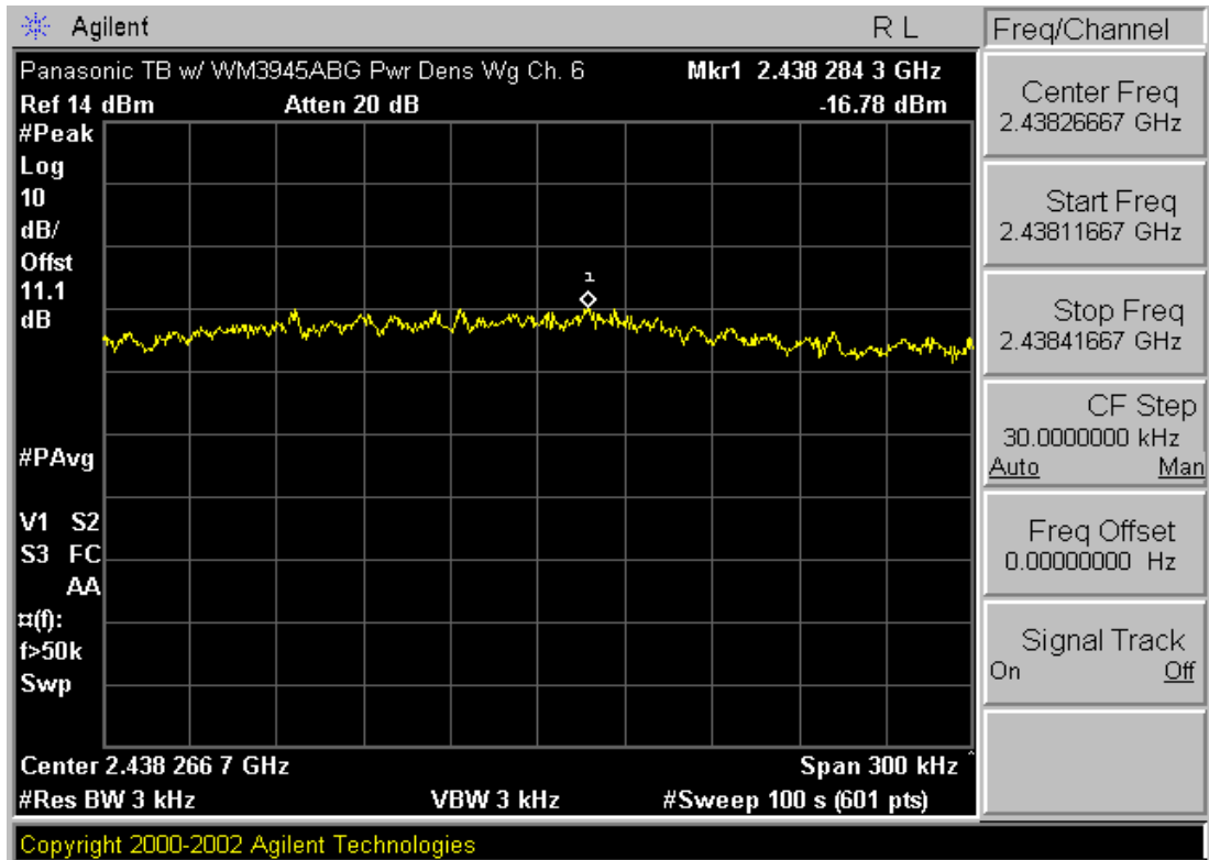
Plot 6-14. Power Spectral Density Plot (802.11g – Ch. 6)
