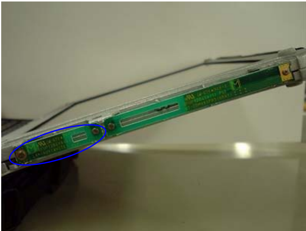
WLAN Aux TX/RX Antenna
