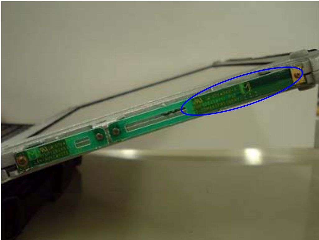
HSDPA TX/RX Antenna
