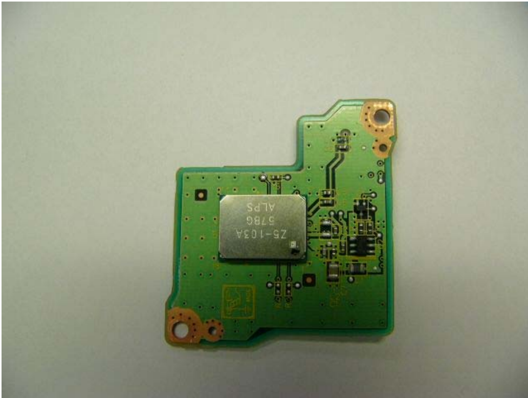
Top View of Daughter Board with Bluetooth Module
