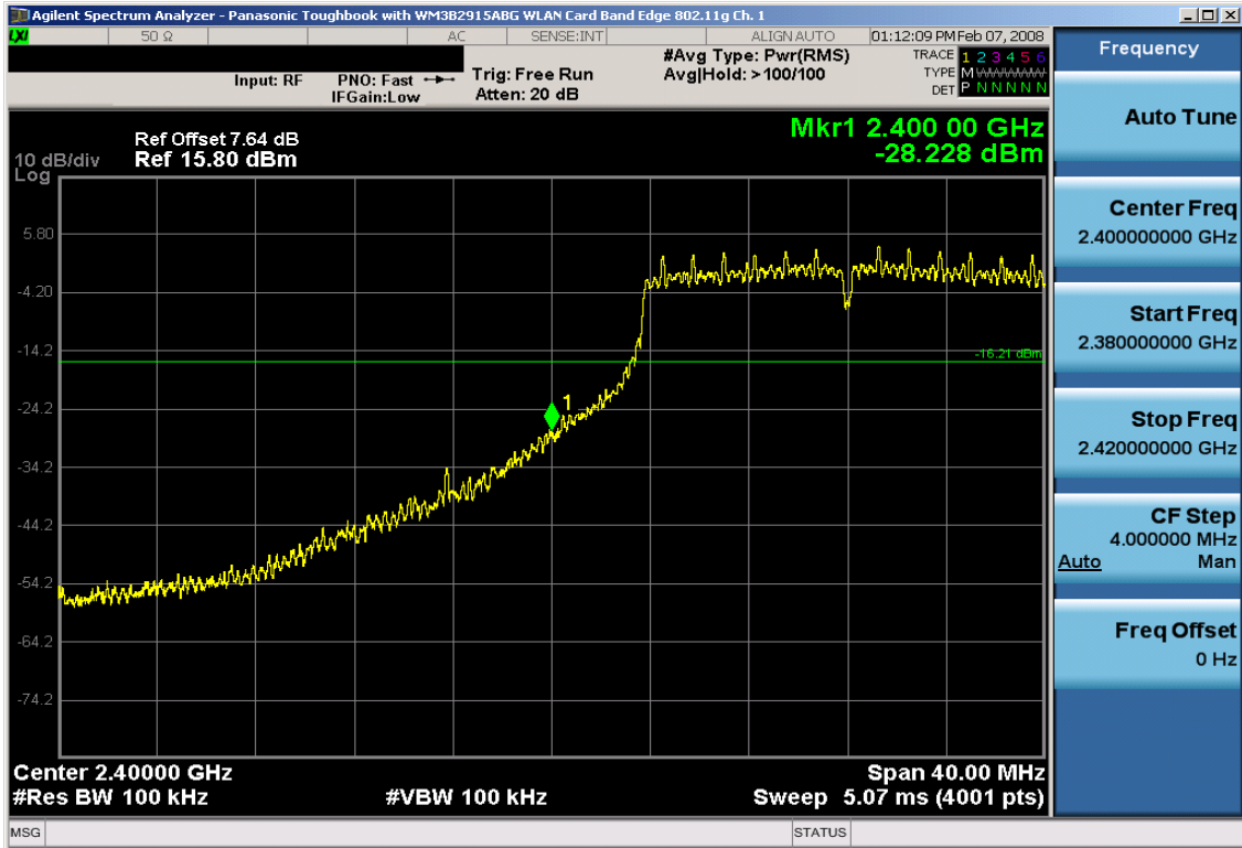
Plot 6-15. Band Edge Plot (802.11g– Ch. 1)
