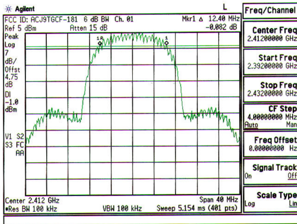
Plot A-1. 6dB Bandwidth Plot – Ch. 01
