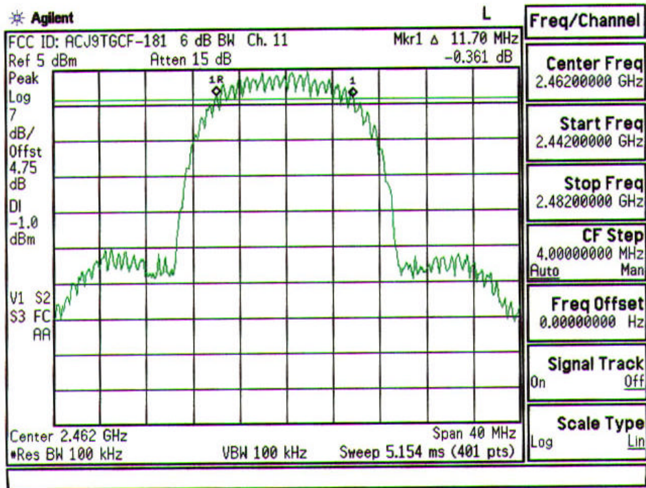
Plot A-3. 6dB Bandwidth Plot – Ch. 11
