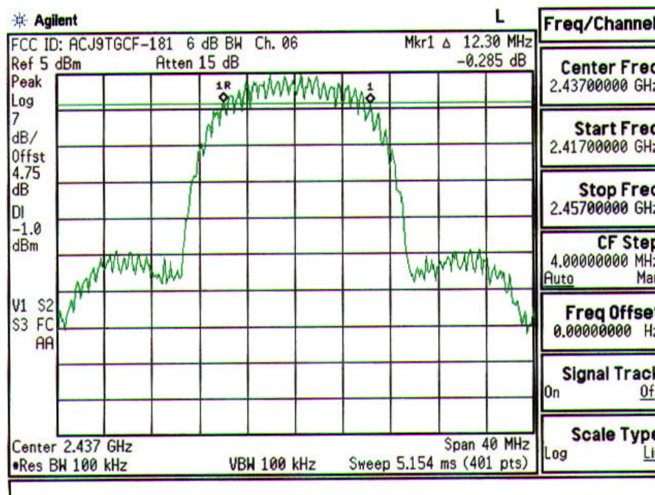
Plot A-2. 6dB Bandwidth Plot – Ch. 06
