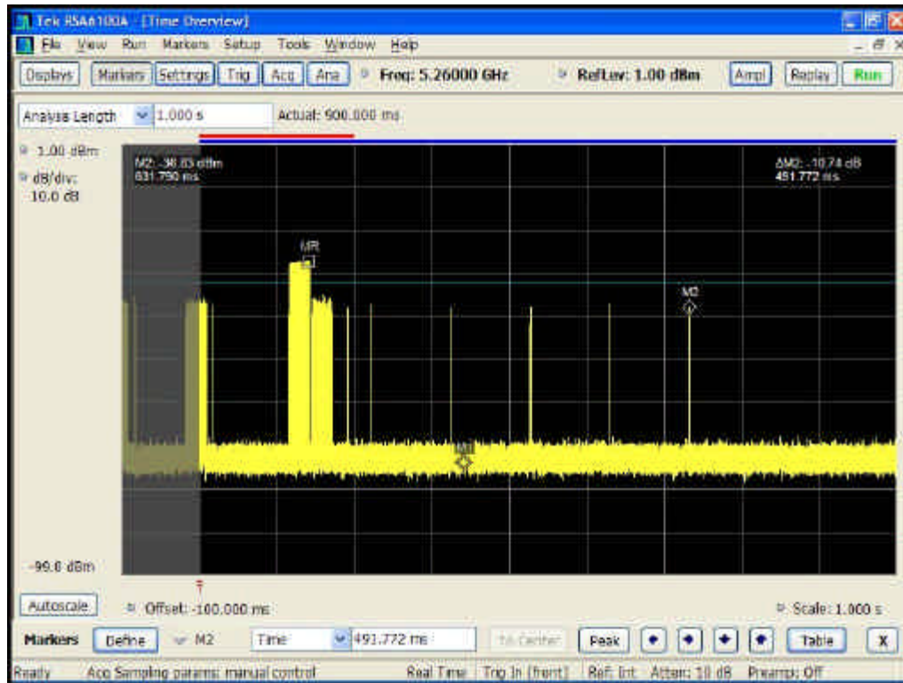
Figure 7: Channel Closing Transmission Time, Aggregate Time After 200ms
