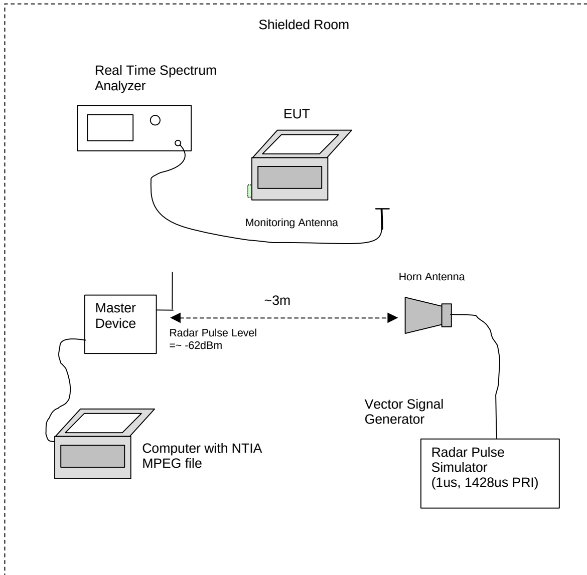
Figure 1: Radiated Test Setup for DFS
