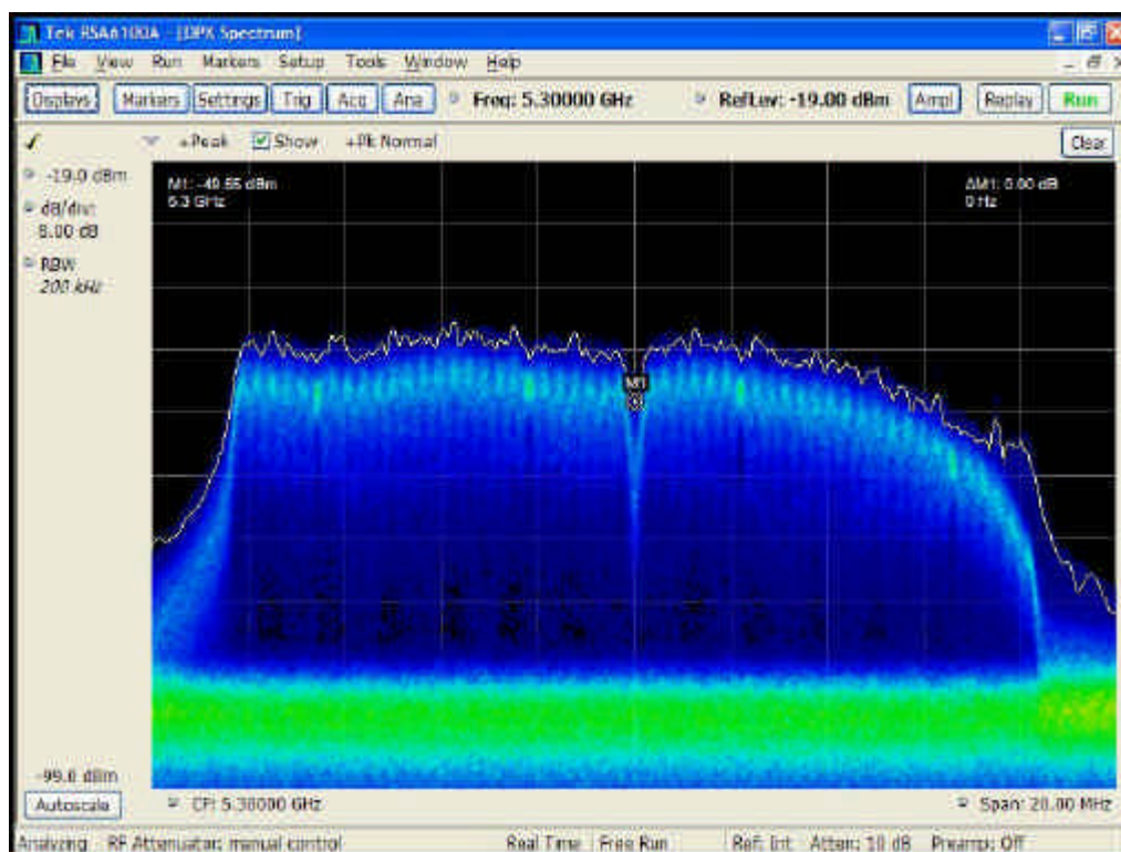
Figure 5: Real-Time Spectrum Display, WLAN Traffic (Streaming Video)
