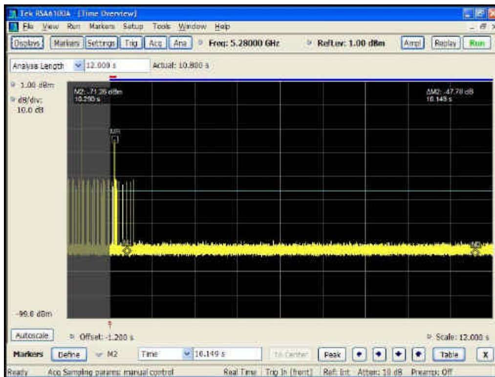
Figure 6: Channel Move Time (<10sec)
