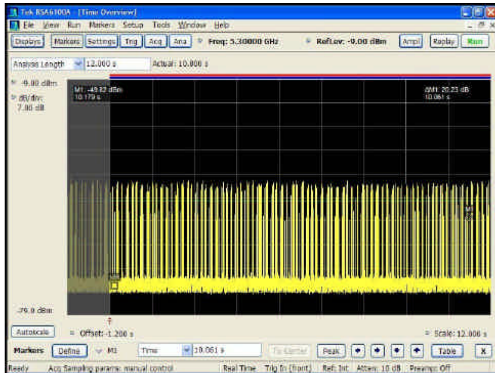
Figure 3: Time Display WLAN Channel Traffic (Streaming Video)
