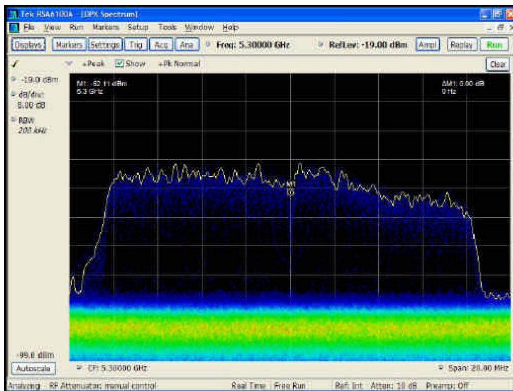
Figure 4: Real-Time Spectrum Display, No WLAN Traffic
