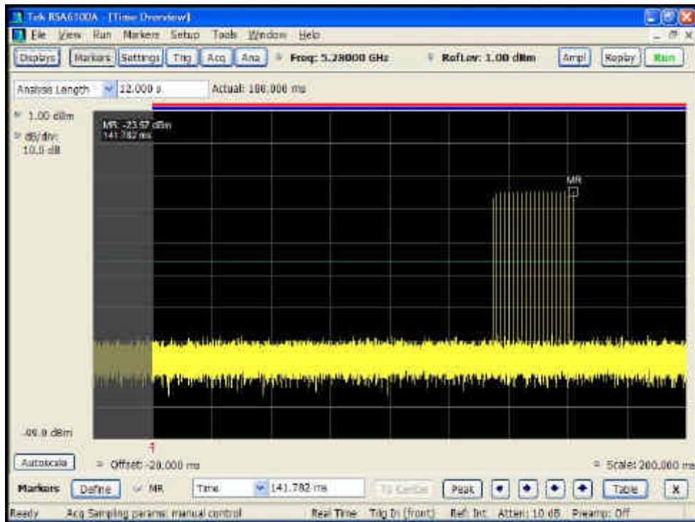
Figure 2: Type 1 Radar Pulse
