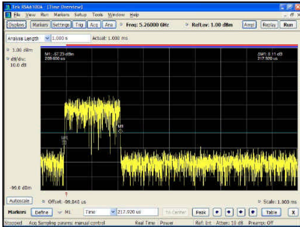
Figure 8: Pulse Width After 200ms
