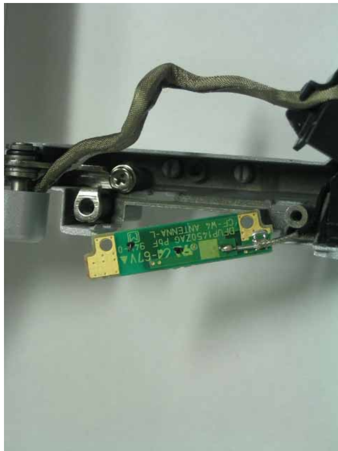
Aux TX/RX Antenna Magnified View(Reverse side)
