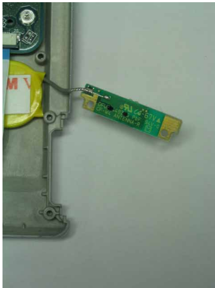
Main TX/RX Antenna magnified View(Reverse Side)
