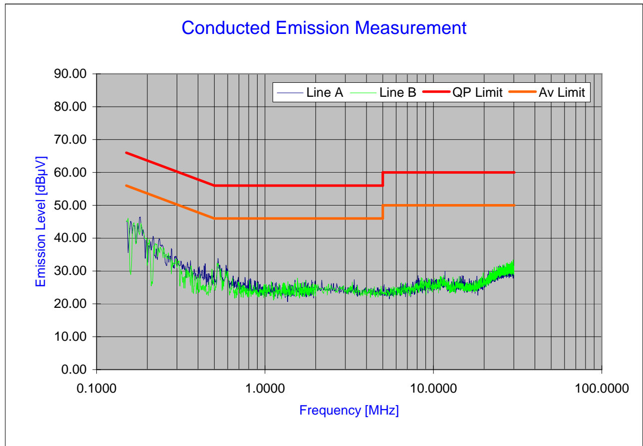
Plot 6-29. Line Conducted Plot with 802.11g
